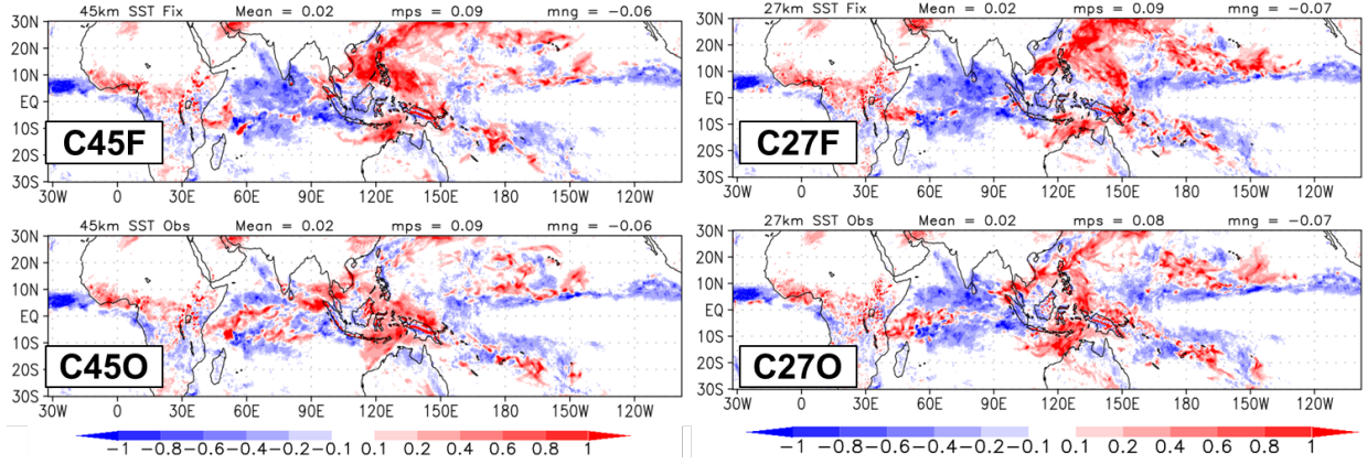
Figure 2: Average precipitation error ( \text{mm hr}^{-1} ), using TRMM precipitation as verification, for COAMPS precipitation for 16-30 November for the 45km simulations (left panels) and 27 km simulations (right panels) with fixed SST (top) and observed SST (bottom).
