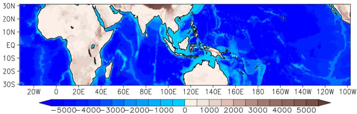
Figure 1: Domain of the COAMPS grid with topography (m).
