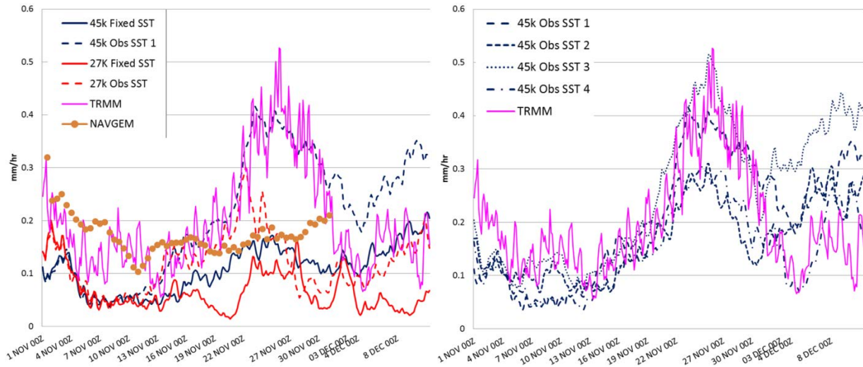
Figure 5: Time series of precipitation ( \text{mm hr}^{-1} ) over the tropical Indian Ocean for TRMM observations (pink) and model simulations as denoted in key.
