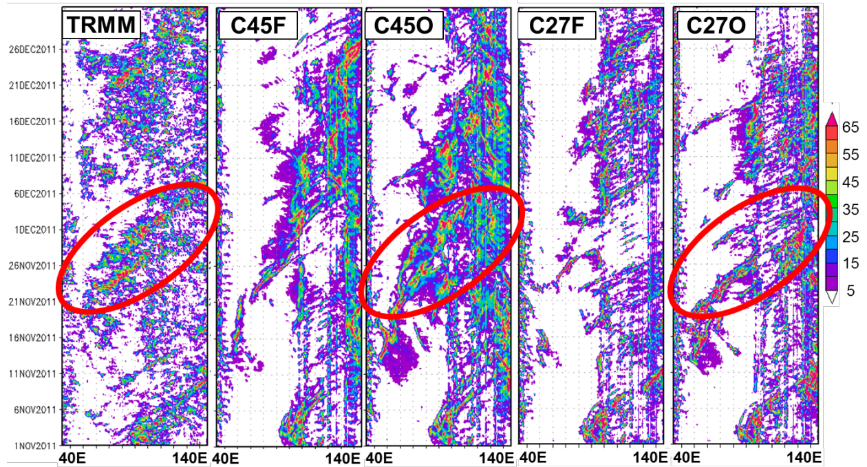
Figure 4: Time-longitude diagrams of precipitation ( \text{mm day}^{-1} , scale given by color bar) from 40 E to 140 E, averaged between 5 S and 5 N, from 1 November through 30 December (time increases along the y axis) for TRMM (left) and C45F, C45O, C27F, and C27O simulations.
