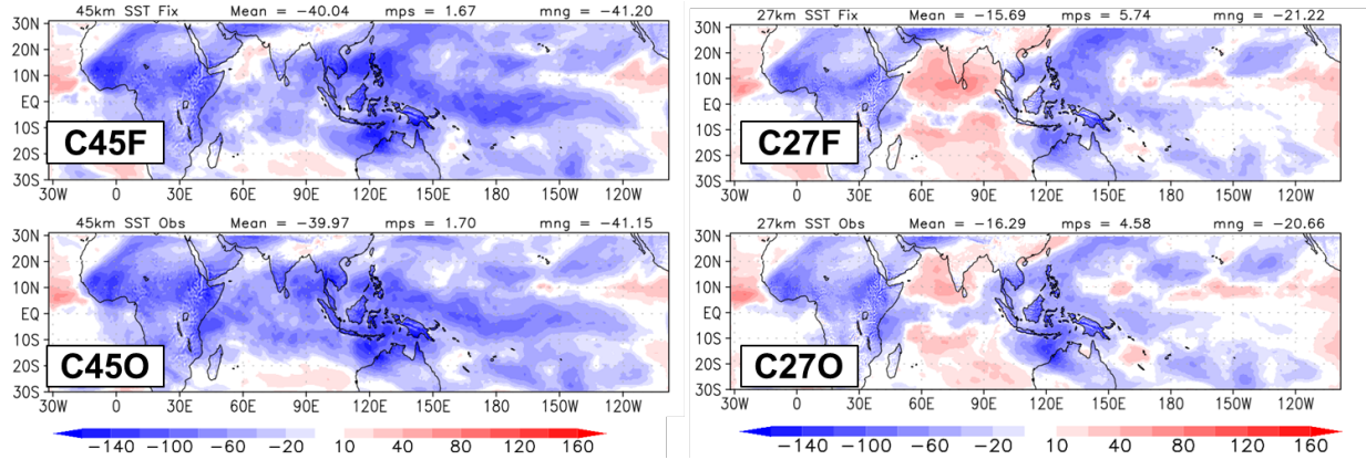
Figure 3: Average OLR error ( \text{W m}^{-2} ) for COAMPS precipitation for 16-30 November for the 45km runs (left panels) and 27 km rms (right panels) for the fixed SST (top) and observed SST (bottom) simulations.
