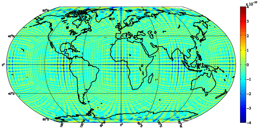
Figure 4: Vertical velocity (m/s) at a height of \sim 2.5 km after 12 hours of integration. The atmosphere is initially at rest, with no topography.
