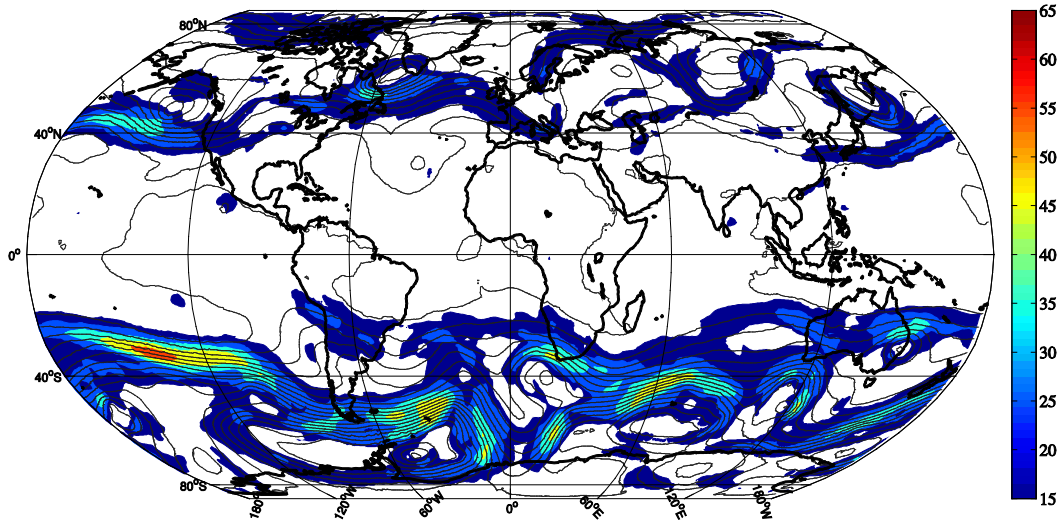
Figure 5: The wind speed (filled contours, starting at 15 m/s, c.i. 10 m/s) and geopotential height (black contours, c.i. 60 m) at 500 hPa at the initial time. Fields are interpolated from 2013062500 NAVGEM fields.
