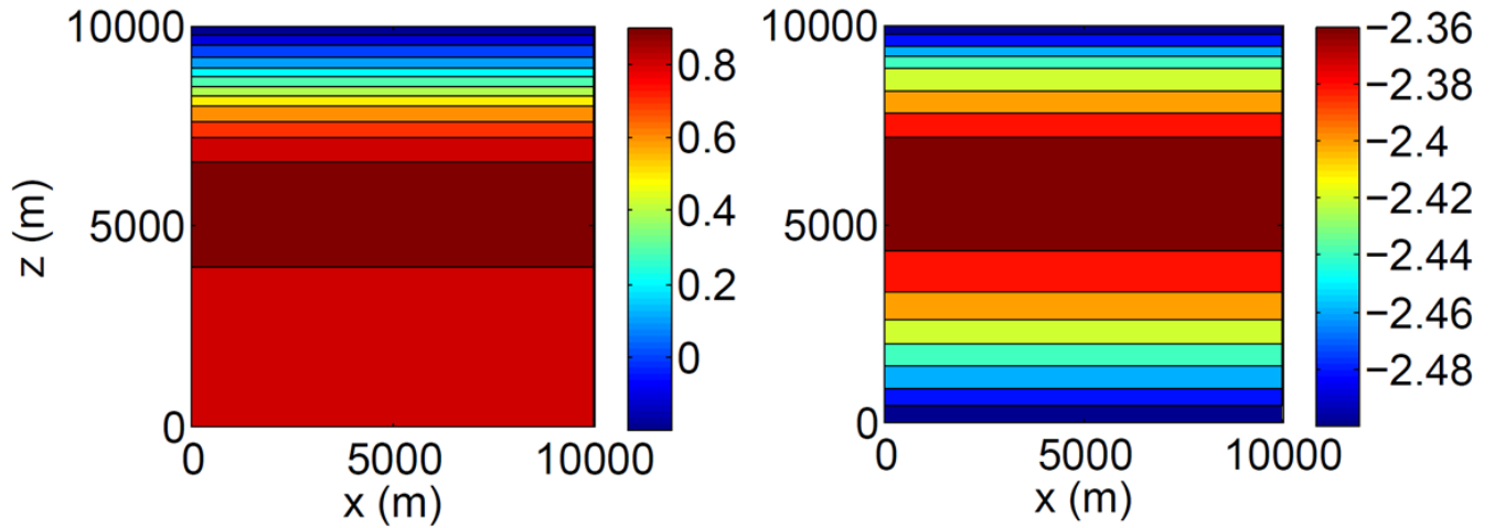
Figure 2: Vertical distribution of the potential temperature perturbation (K) after 24 hours using the radiation parameterization. Effects of the shortwave warming (left panel) and longwave cooling (right panel) are shown separately.
