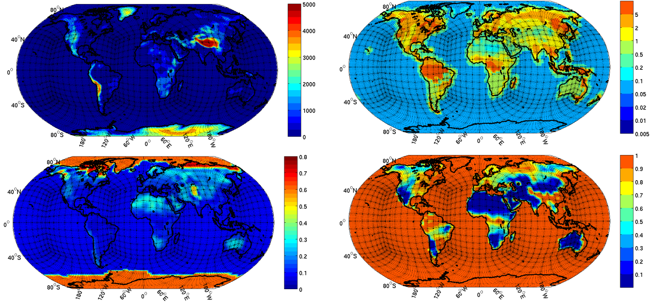
Figure 3: Topography (top left, in meters), surface roughness (top right, in meters), albedo (bottom left, no units), and ground wetness (bottom right, no units) on a cubed-sphere mesh. The average horizontal spacing of nodal points (black color dots) is approximately 100 km.
