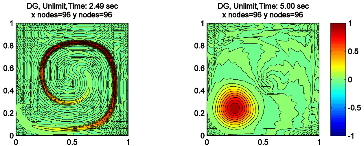
Figure 6: Tracer concentration at half time (left panel), when it is maximally stretched, and final time (right panel). Courtesy of prof. Dale Durran (UW).
