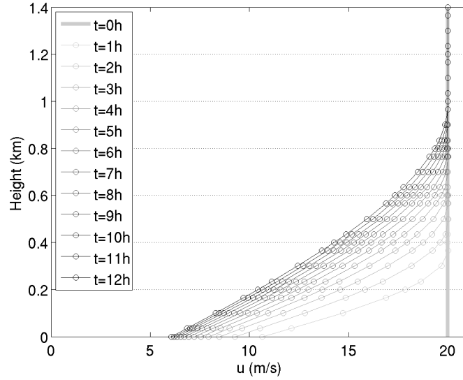
Figure 1: Evolution of the vertical wind profile with time for the first twelve hours with the surface fluxes turned on. The atmosphere is neutrally stratified.
