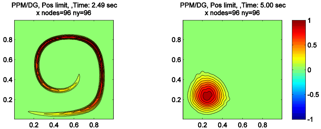
Figure 7: Tracer concentration at half time (left panel), when it is maximally stretched, and final time (right panel), when using PPM in the vertical direction. Courtesy of prof. Dale Durran (UW).
