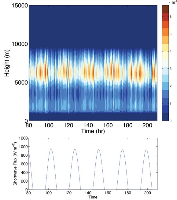
Figure 4. Horizontally averaged cloud water content from the low resolution simulation (top) and surface shortwave radiation (bottom).
