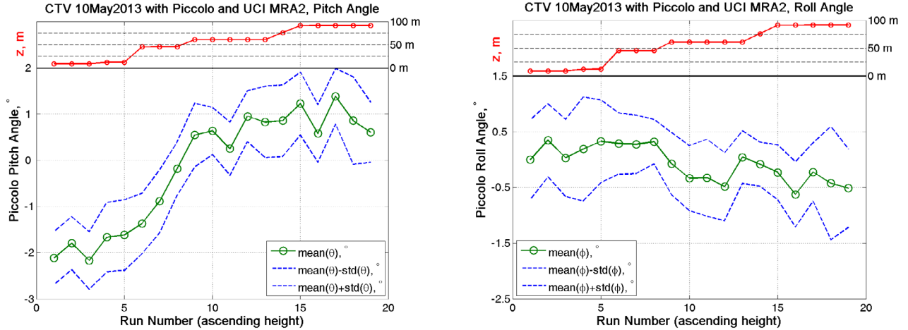
Figure 11: CTV Pitch angle, \theta , (left) and roll angle (right) from Piccolo autopilot for all 19 straight and level runs: means (green circles and line), \pm 1 \sigma (blue dashed lines). The runs are sorted and numbered from lowest to highest altitudes. The top red line and circles represent the MRA2 run means with their associated axis on the top left. The CTV pitches down 3^\circ more at the lowest runs but the pitch angle standard deviation remains small ( 0.7^\circ ) and is about the same for all runs. This is a crucial and a huge improvement compared to the original (2007/2008) Meggitt control system. The roll angle is very small and remains within \pm 0.5^\circ .
