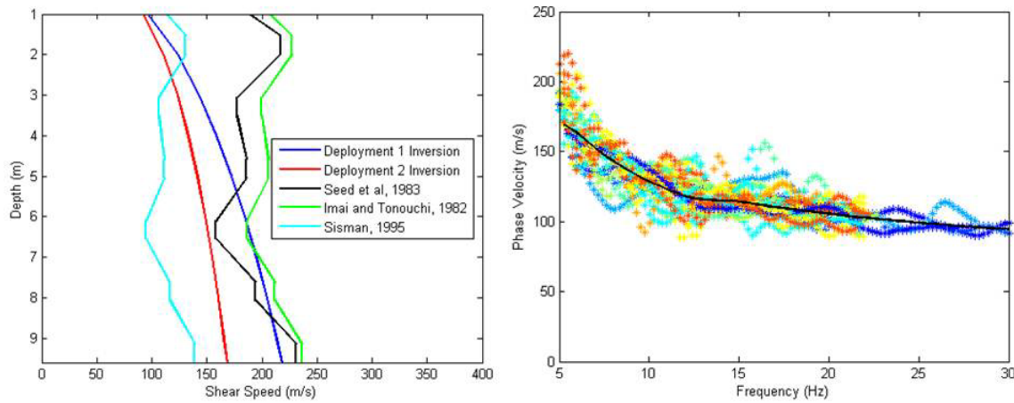
Figure 4: Comparison of the shear speed profiles (left panel) estimated for Deployment 1 and Deployment 2 at the Davisville site with the range of shear speed values estimated from the SPT blow counts (using three different methods) contained in boring log BH-15. Right panel shows the theoretical dispersion (black line) calculated using Godin-Chapman model for the inverted shear speed profile compared with the data. The different geophone pairs are represented by the different colors.
