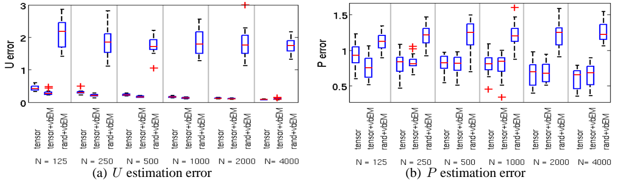
Figure 5.4: Simulation confirming consistency of the proposed algorithm
