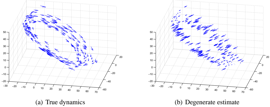
Figure 3.1: Degenerate estimate by the unordered approximation on 200 data points
