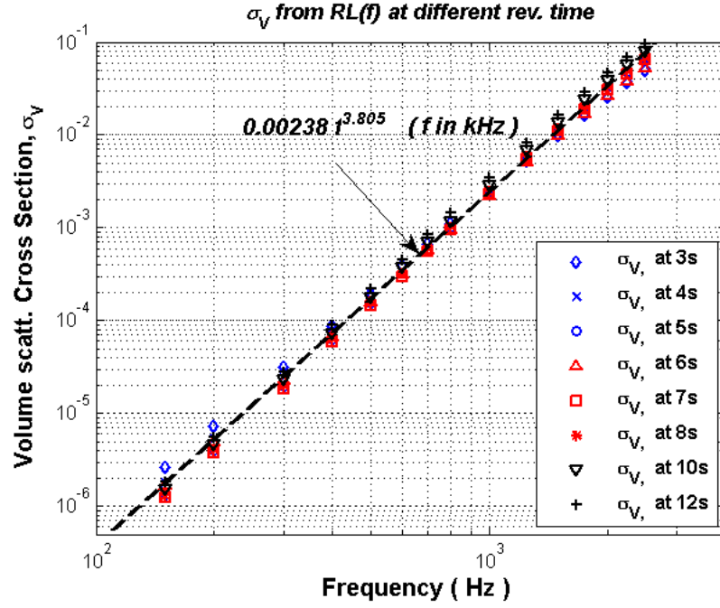
Fig. 3 The sediment volume scattering cross section, inverted from long-range reverberation data at the ASIAEX site, exhibits strong frequency dependence: \alpha_V = 0.00238 f^{3.805} ( f in kHz)
