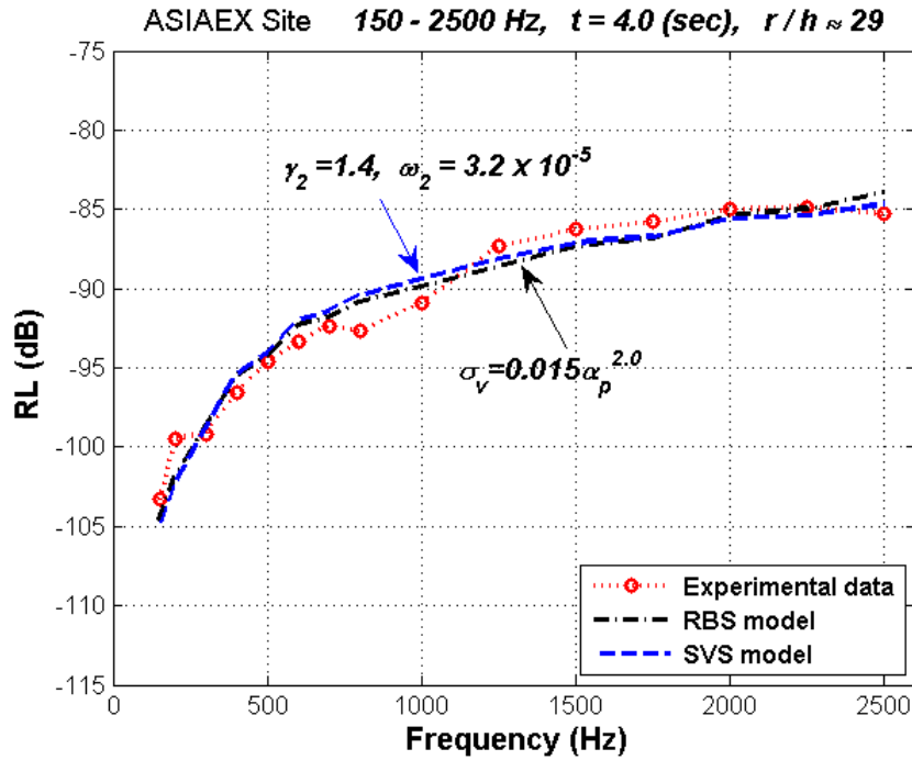
Fig. 2. Wideband reverberation data at the ASIAEX site are used to invert a set of seabed scattering parameters for the RBS and SVS models.
