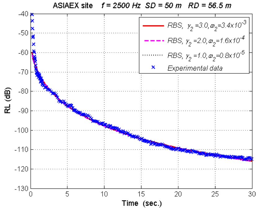
Fig. 1. Internal parameter coupling between the spectral exponent \gamma_2 and the spectral strength \omega_2 for the RBS model. Three different pairs of \gamma_2 and \omega_2 result in a identical RL(t) . An increase in \gamma_2 can be compensated for by an increase in \omega_2 .
