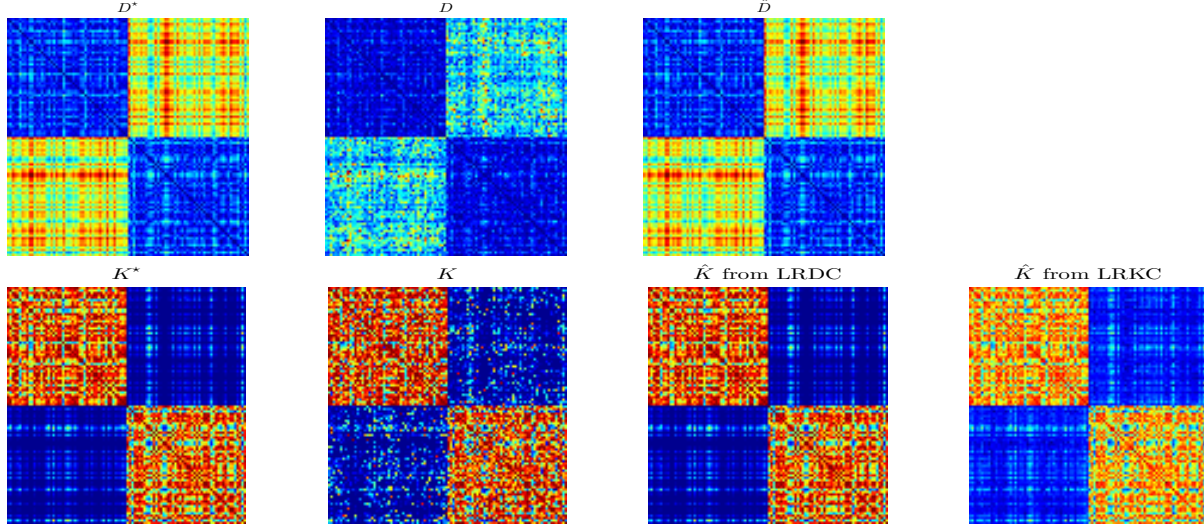
Figure 6.2: Example results from LRKC and LRDC. K^* and D^* are the groundtruths. K and D are the noisy observations. \hat{K} and \hat{D} are the low-rank results produced by LRKC and LRDC.
