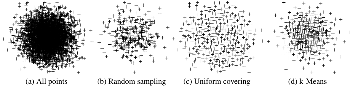
Figure 7.1: Condensing results of a 2D standard Gaussian point set using different condensers.
