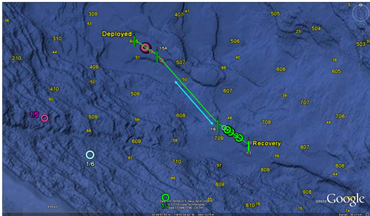
Figure 1. Eight encounters detected by the ERMA detector with ICI=0.2-0.7 . ICI=0.2-0.7 is the optimum and produced the best match to the manually-derived and the M3R detections record.
