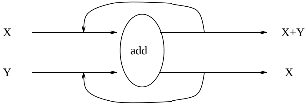
Figure 3.8: A data-flow diagram for computing the Fibonacci stream
