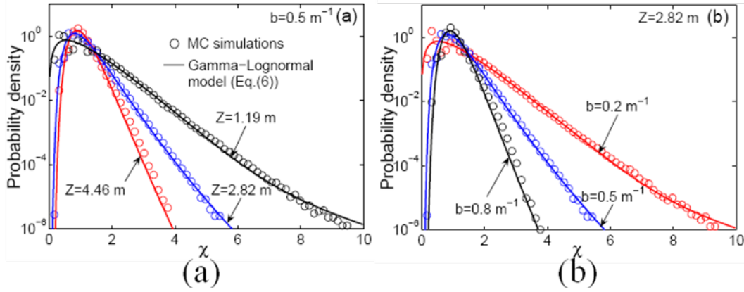
Figure 2. Performance of the Gamma-Lognormal mixture model for the PDF of the normalized average intensity compared to Monte Carlo RT simulation predictions, under a ECKV wave surface of MSS=0.77 and water attenuation coefficient c=1\text{m}^{-1} . (a) Scattering coefficient b=0.5\text{m}^{-1} for different depths Z=1.19, 2.82, 4.46\text{m} , the corresponding model parameter values are \sigma=0.4564, 0.1479, 0.0806 ; and \mu=0.923, 0, 0 . (b) Depth Z=2.82\text{m} for different scattering coefficients b=0.2, 0.5, 0.8 \text{ m}^{-1} , the corresponding model parameter values are \sigma=0.4762, 0.1479, 0.0728 ; and \mu=0.950, 0, 0 .
