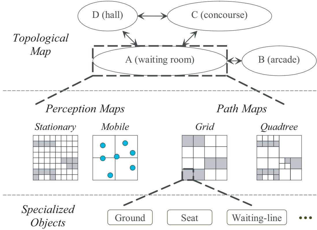
Figure 3.2: Hierarchical environment model.
