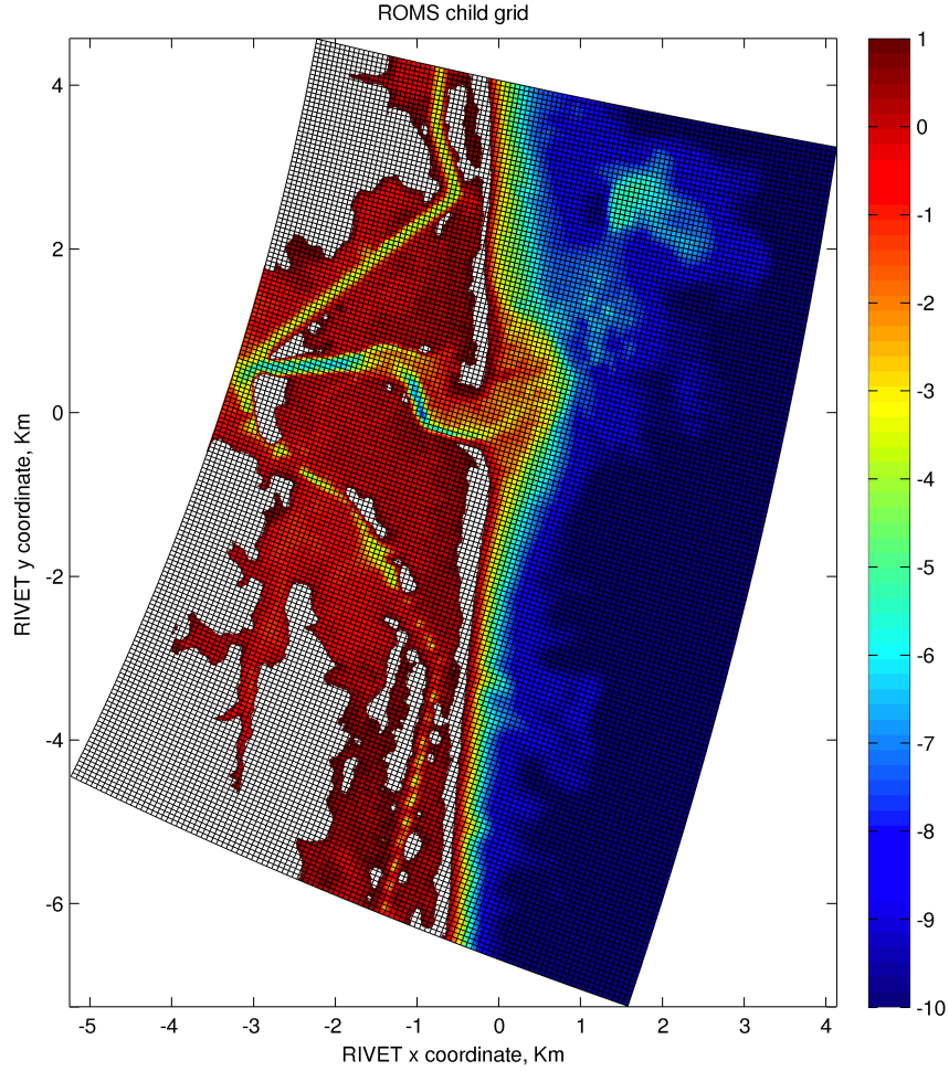
Figure 4: Map of the COAWST (SWAN/ROMS) model grid for the New River Inlet region. Bathymetry is colored (see scale at right) and the land mask is in white. Grid spacing varies between 10–15 m.
