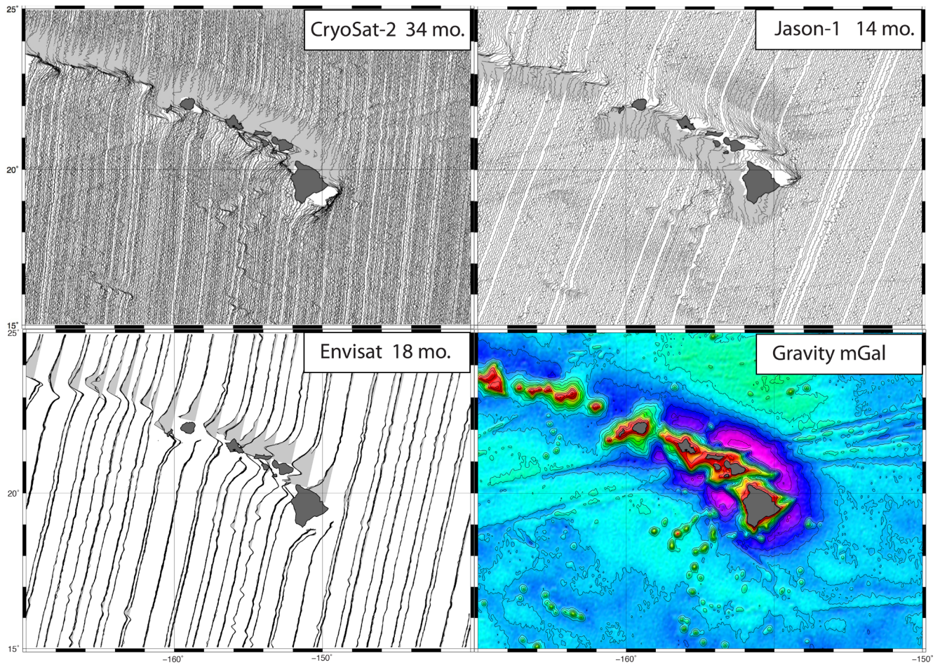
Figure 1. Along track sea surface slope from CryoSat, Envisat, and Jason-1. The along-track slopes from all satellites, both ascending and descending directions, are combined using a biharmonic spline method to produce north and east sea surface slope maps and ultimately gravity anomaly (lower right).
