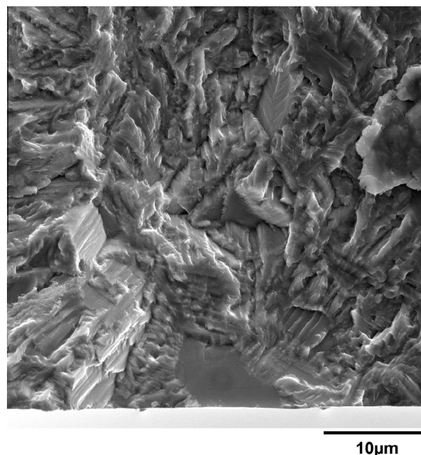
Fig. 4. Typical fatigue crack origin (lower edge) showing a single, surface-connected, alpha grain facet where crack nucleation occurred.
