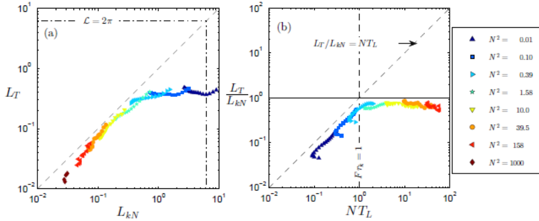
Figure 2: Turbulent kinetic energy length scale, L_{kN} , versus Thorpe scale, L_T : (a) direct comparison, and (b) plotted against the dimensionless stratification parameter, NT_L .
