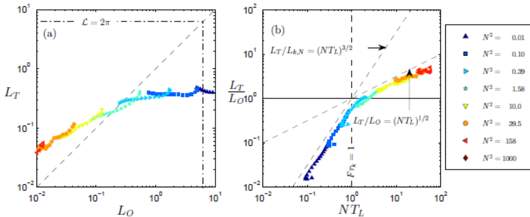
Figure 1: Ozmidov length scale, L_O , versus Thorpe scale, L_T : (a) direct comparison, and (b) plotted against the dimensionless stratification parameter, NT_L .
