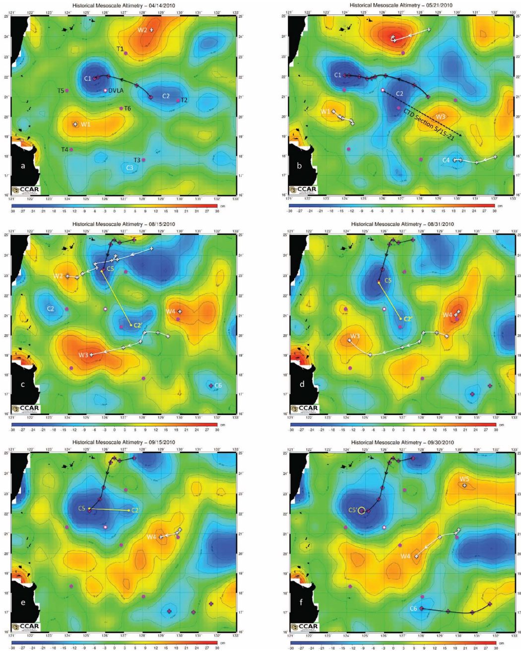
Figure 1. The distribution of cyclonic (cold, blue) and anticyclonic (warm, red) mesoscale eddies in the PhilSea10 array region. The mooring locations T1-T6 and DVLA are indicated in panel a. The same situation is revisited 37 days later in panel b, with eddy tracks superimposed. Warm eddy tracks are shown in white and cold eddies in black. The distance between “x’s” is the distance traveled in 14 days and thus is an indication of relative eddy propagation speed. Panel b also shows the CTD/ADCP transect location for Figure 2. Panels c-f show an eddy/eddy interaction plus additional representative eddy tracks. See text for additional details. (Base maps from the Colorado Center for Astrodynamic Research, CCAR)
