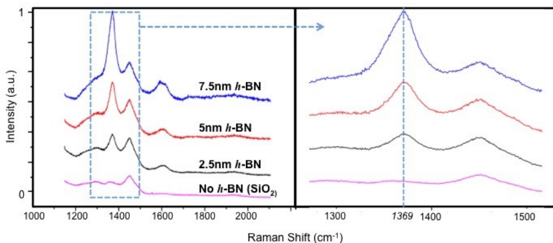
Figure 4.9: Figure 4.8 with the redundant single layer Site 2 Raman spectra removed. Note on the right-hand magnified region that all 3 of the h\text{-BN} spectra show no shifting of the 1367\text{ cm}^{-1} E_{2g} peak with a change in thickness (seen here at 1369\text{ cm}^{-1} due to possible material strain or system calibration shifting).
