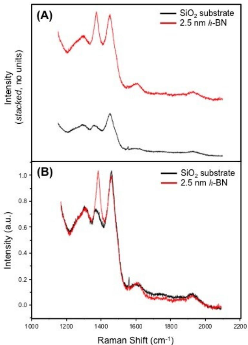
Figure 4.7: Raman spectra of Site 2 of atomically thin h -BN film on SiO 2 . (A) Pt 1, Black: hole in the h -BN film revealing the SiO 2 substrate; Pt 2, Red: single layer of h -BN film 2.5 nm thick (7 atoms). (B) Depiction of chart A normalized to the h -BN peak. [Spectra was obtained after 30 accumulations of 60 second exposures using a 488 nm Argon ion laser with 1.12mW measured power at sample with 20μm slits, 100X objective, 3000 lines/mm grating centered at 1650 cm -1 ]
