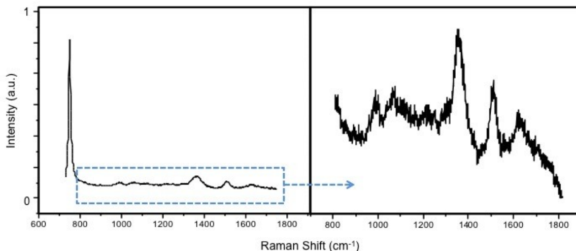
Figure 3.4: Side-by-side comparison of h -BN on sapphire spectra demonstrating the effects of preferentially centering gratings. (LEFT) Note that when the 3000 line/mm grating is centered at 1264 \text{cm}^{-1} the characteristic \text{Al}_2\text{O}_3 peak at 750 \text{cm}^{-1} drowns out the relatively weak 1367 \text{cm}^{-1} h -BN peak. Longer dwell times necessary for h -BN returns can often overload the CCD. (RIGHT) when the same 3000 line/mm grating is centered at 1336 \text{cm}^{-1} the \text{Al}_2\text{O}_3 peak is removed from the field-of-view allowing for a more prominent h -BN return.
