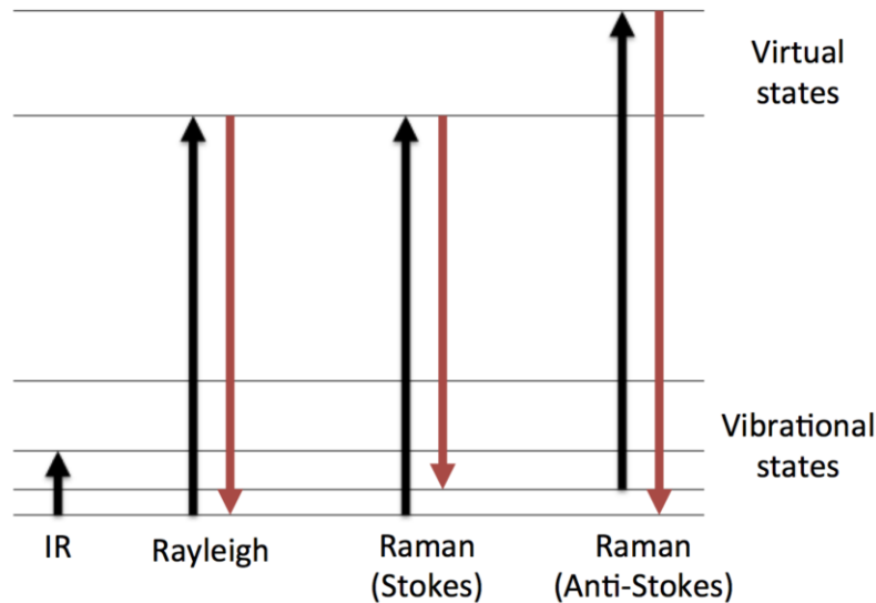
Figure 2.1: Diagram depicting both anti-Stokes and Stokes Raman scattering as compared to Rayleigh scattering and Infrared absorption. Note that the majority of reflected photons, when incident on a surface, return at their original wavelength because these photons interact elastically with the sample material. However, every 1:1,000,000 photons incident on a surface will interact inelastically with the material due to phonon-coupling and will be scattering at either a higher frequency (anti-Stokes) or at a lower frequency (Stokes). Through the analysis of this shift a great deal of information concerning a material's rotational and vibrational modes can be understood.
