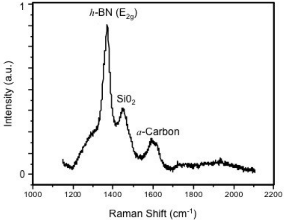
Figure 2.2: Raman spectra of h -BN with the 1367\text{ cm}^{-1} E 2g peak labeled [15]. A lower intensity and broader peak around \sim 1600\text{ cm}^{-1} was attributed to the G and D' peaks of carbon introduced to the system through the transfer process via thermal release tape [35]. The 1448\text{ cm}^{-1} peak is attributed to a higher order SiO 2 combination peak given that it also appears in Raman analysis of pure SiO 2 wafers.
