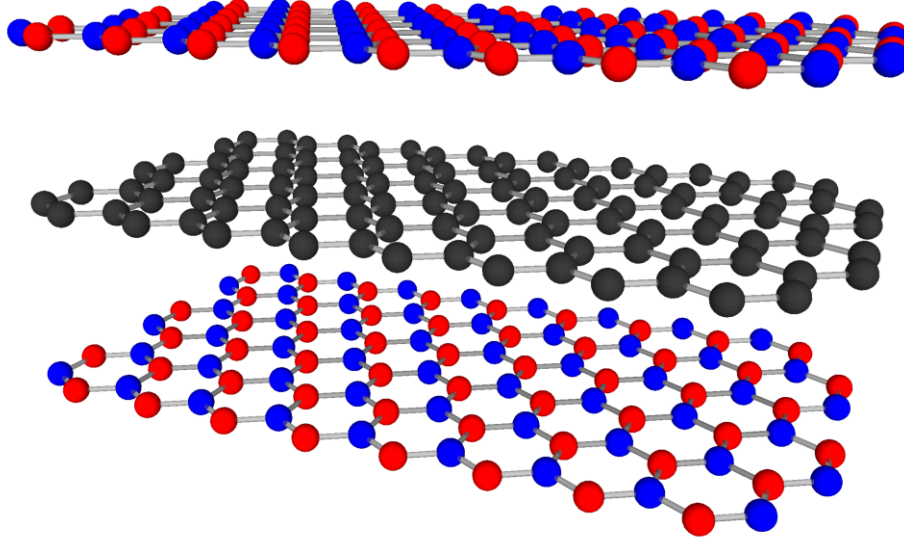
Figure 1.1: Currently, only graphene on a h -BN substrate has been shown to preserve graphene's mobility of 100,000 \text{ cm}^2/\text{Vs} [9]. The two lattices have only a 1.7% mismatch and complimentary hexagonal planar structures with weak inter-planar bonding allows h -BN to insulate graphene from thermal phonon interactions which would otherwise cause electron scattering and degradation of graphene's high electron mobility.
