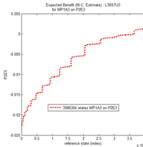
Figure 8.19 Max-Plus Probability Solution Performance
