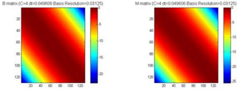
Figure 7.1 Analytically computed B and M matrices for a 1-D LQR problem: left panel shows the B matrix and right panel shows the M matrix
