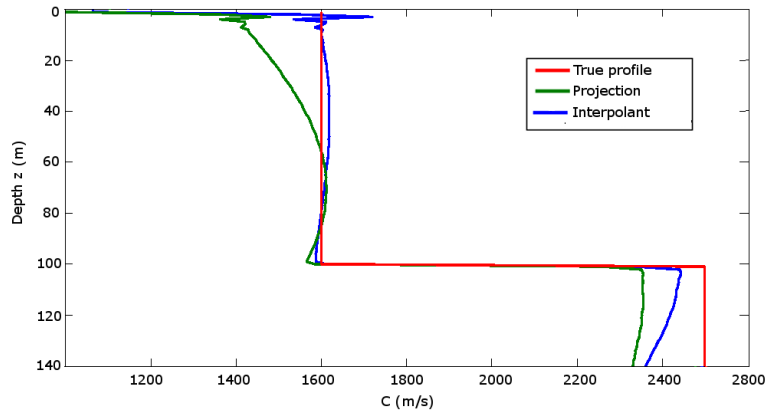
Figure 4: Sediment sound speed estimation with an analytic method, improving on results previously obtained from similar techniques.
