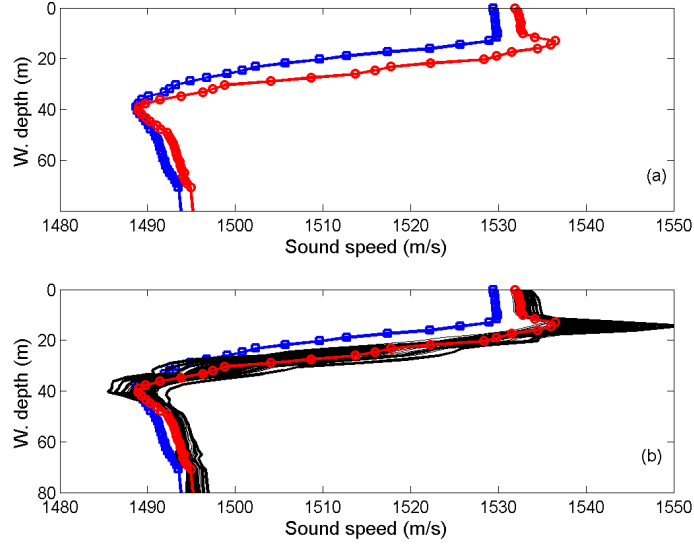
Figure 2: (a) The mean sound speed profile as calculated by the CTD measurements (squares) and the sound speed profile constructed with the MAP estimates obtained from the extracted arrival time PDFs (circles). (b) The profiles of (a) with superimposed sound speed profiles constructed from distinct arrival time particles (solid curves).
