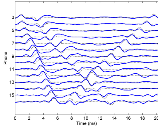
Figure 3: Real data (solid lines) and synthetic time-series (dotted lines) generated using the linearization estimates.
