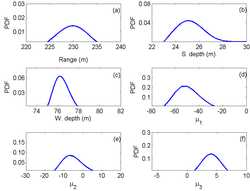
Figure 1: PDFs of (a) source range, (b) source depth, (c) water column depth, (d) \mu_1 , (e) \mu_2 , (f) \mu_3 for real data.
