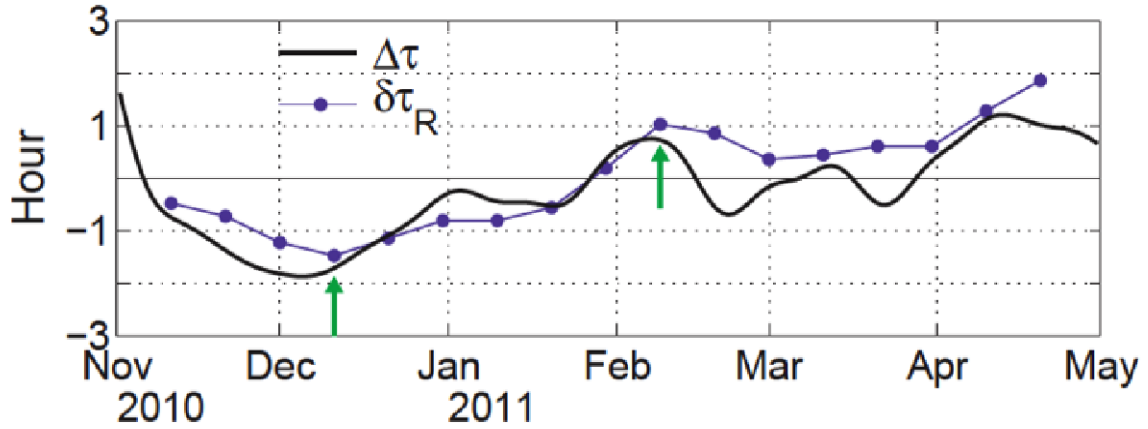
Fig. 6 Comparison of variability in observed wave arrival time ( \Delta\tau ) with predicted values ( \delta\tau_R ) based on ray-trace calculations for the HYCOM simulations.
