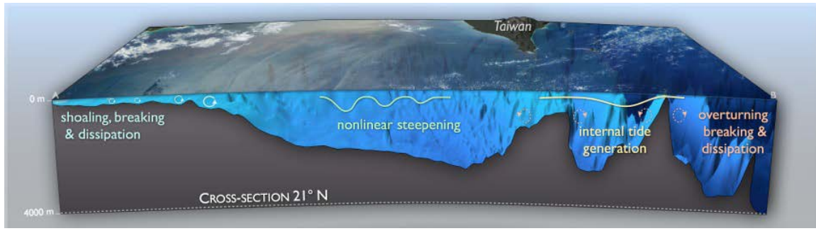
Fig. 1. This contribution to IWISE focused on the generation of internal tides through tidal forcing over the ridges in Luzon Strait and their subsequent nonlinear evolution as they propagate westwards across the deep basin of the South China Sea.
