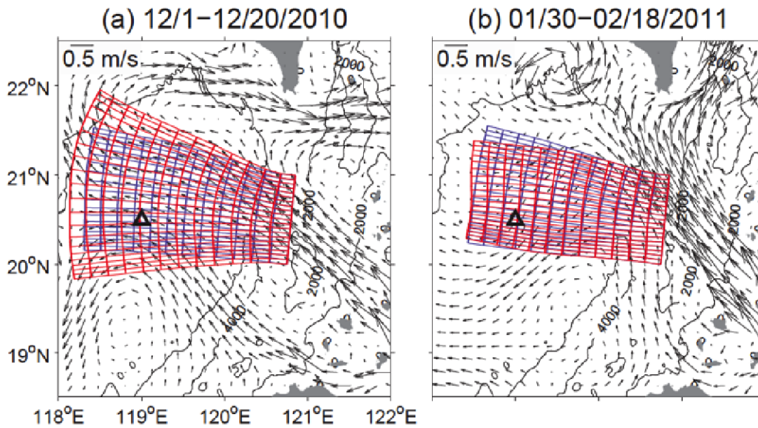
Fig. 7 Ray-trace calculations using the 2-dimensional Taylor-Goldstein equation for internal waves radiated from just west of Luzon Strait, with HYCOM simulated velocity and density fields for periods of (a) strong inflow and (b) weak currents in the deep basin. The \Delta symbol indicates location of P05 PIES observations for the comparisons shown here.
