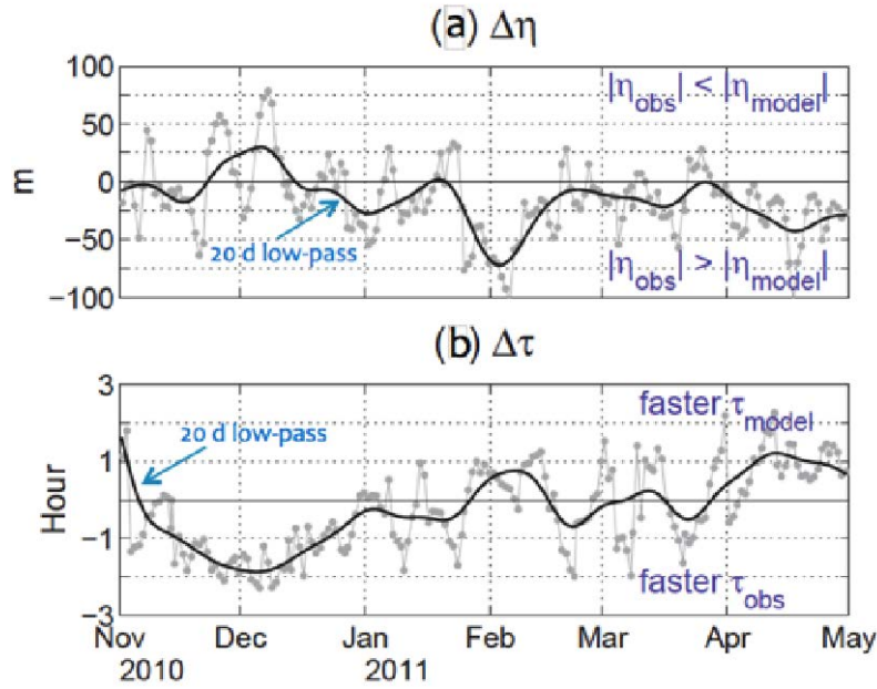
Fig. 3 Time series of the difference between simulated and observed (a) internal wave amplitude and (b) internal wave arrival time.
