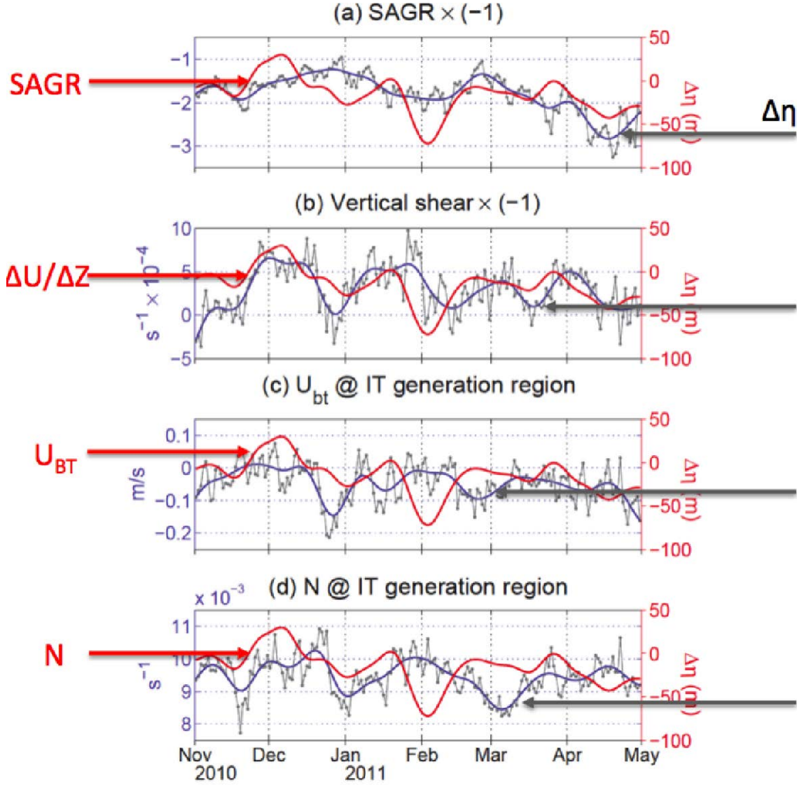
Fig. 5 Comparison of observed internal wave amplitude difference from H-H model simulation with different parameters: (a) Soliton Amplitude Growth Ratio, (b) vertical shear, (c) barotropic forcing, (d) stratification.
