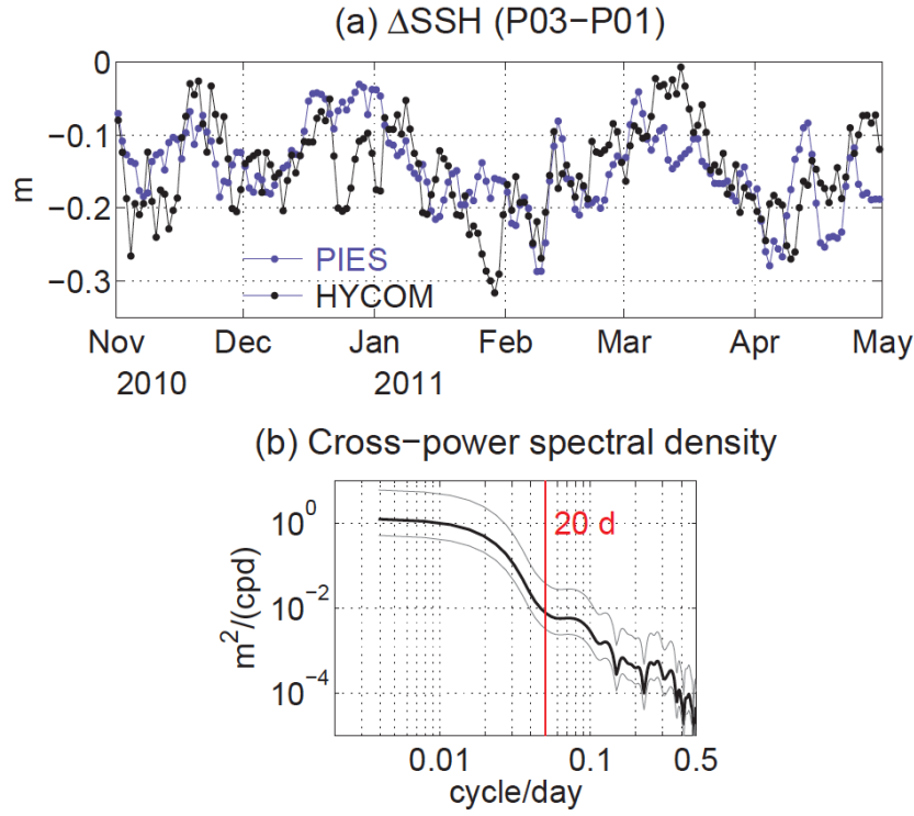
Fig. 2 (a) Comparison of observed fluctuations in sea surface slope \Delta\text{SSH} (blue) with corresponding HYCOM simulation (black). (b): Cross-power spectral density between the observed and simulated time series.
