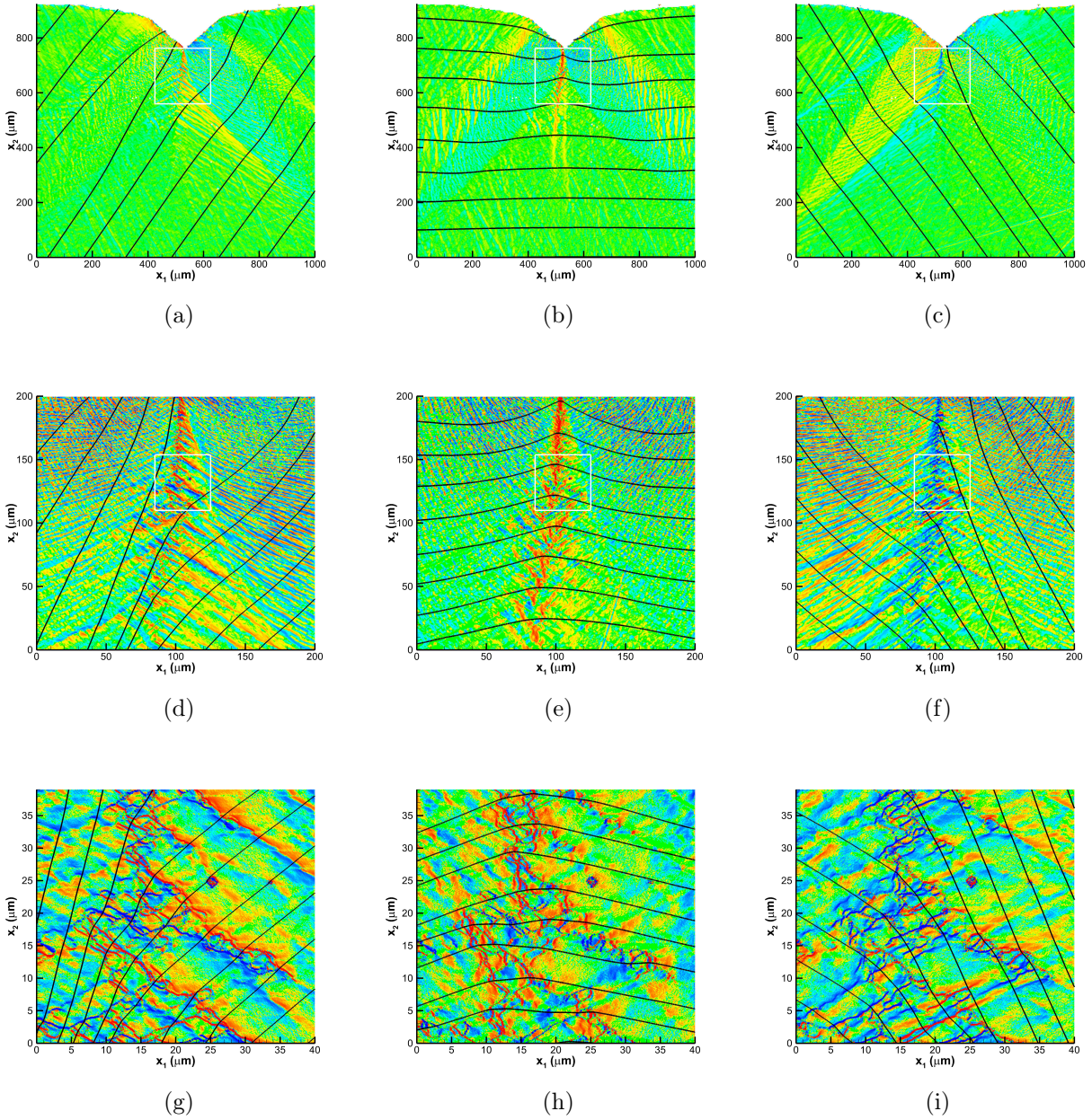
Figure 5: The three columns show GND density distributions on slip pair 1 (left column), slip pair 2 (middle column) and slip pair 3 (right column), with spatial resolutions along the rows of 2500 nm (top row), 500 nm (middle row) and 100 nm (bottom row).
