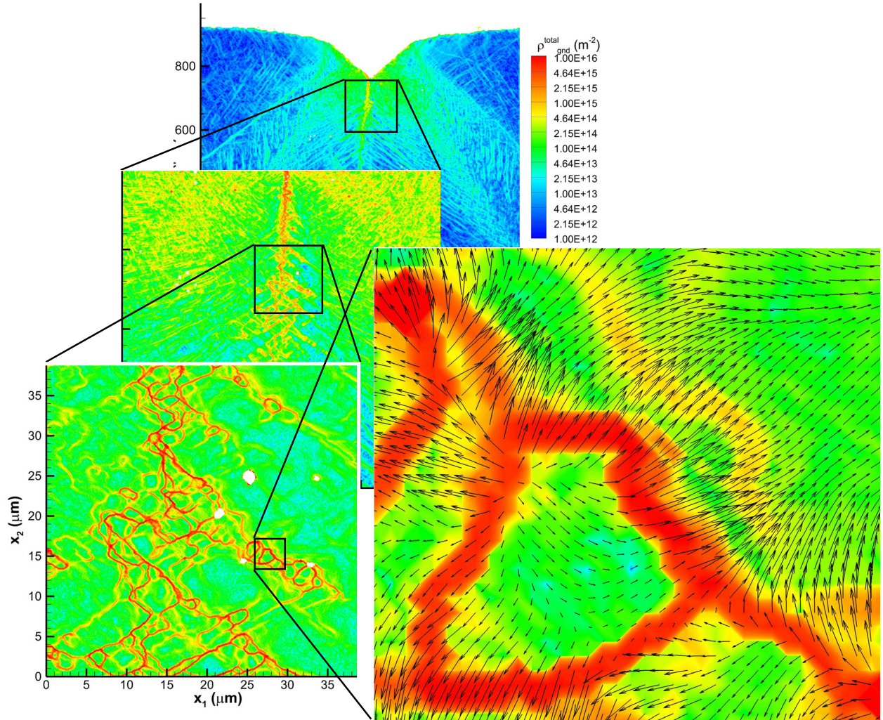
Figure 4: Multiscale perspective of Lower Bound on Total GND Density. The back three images are from the right column of Fig. 3. The Net Burgers Density Vector, \mathbf{B} , is shown on a 100 nm by 100 nm array of deformed material points.
