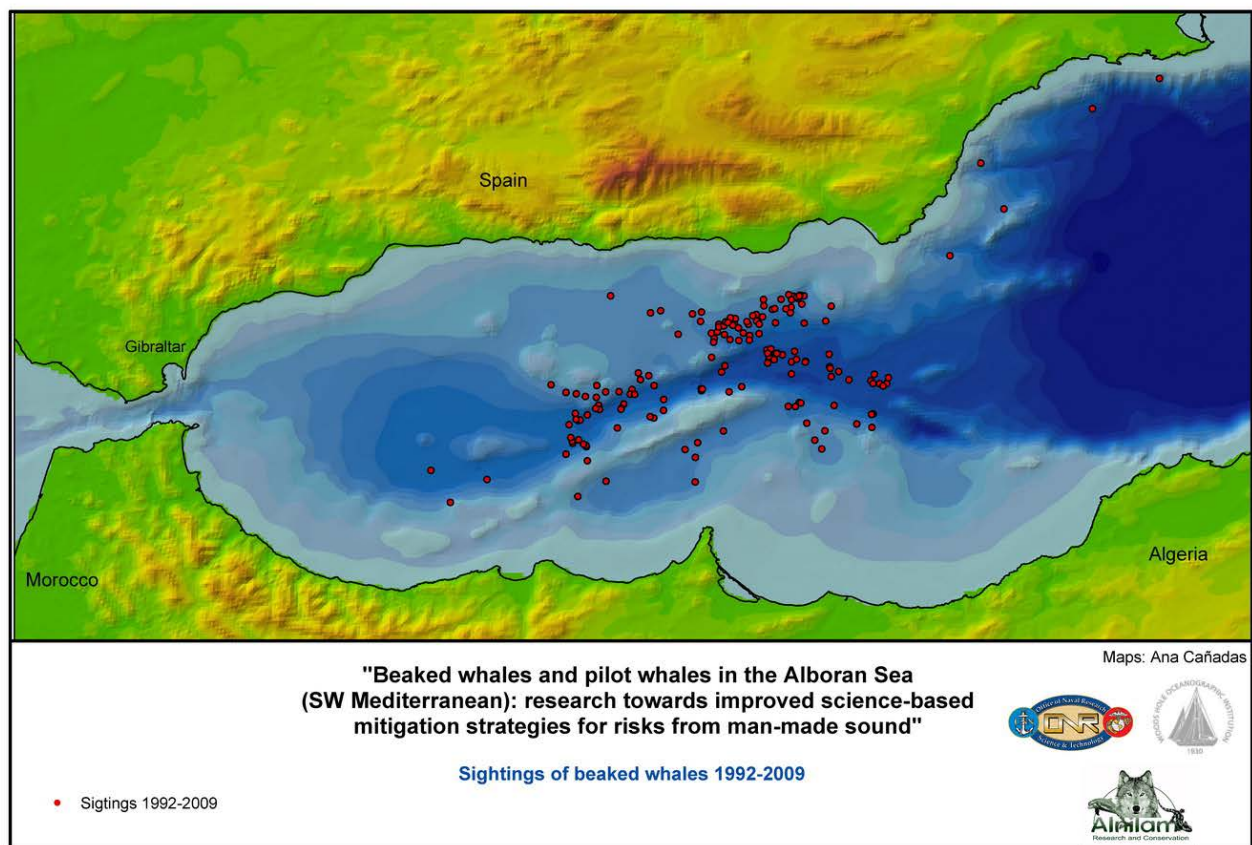
Figure 4. Sightings of beaked whales from 1992 to 2009 by all ships.
