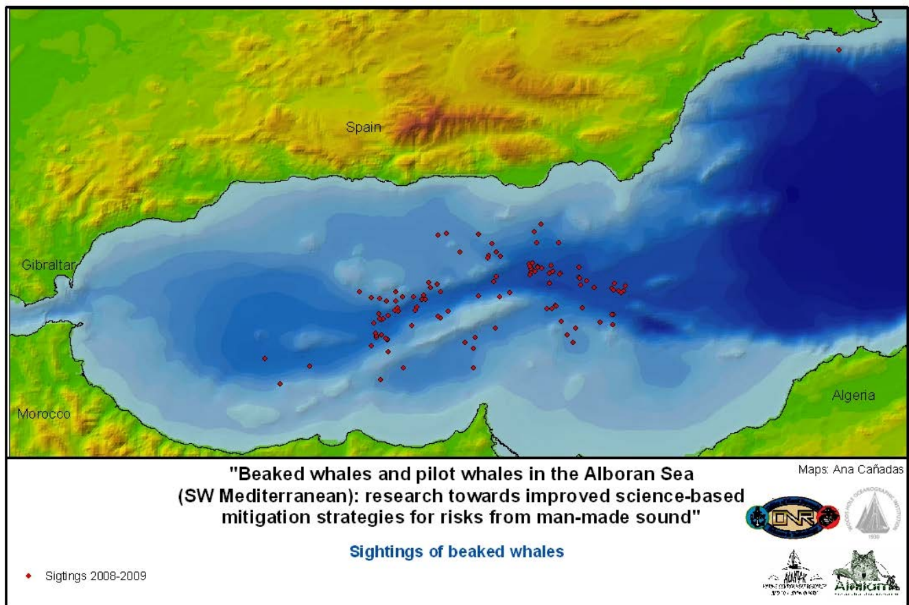
Figure 3. Sightings of beaked whales in 2008 and 2009 by all ships.
