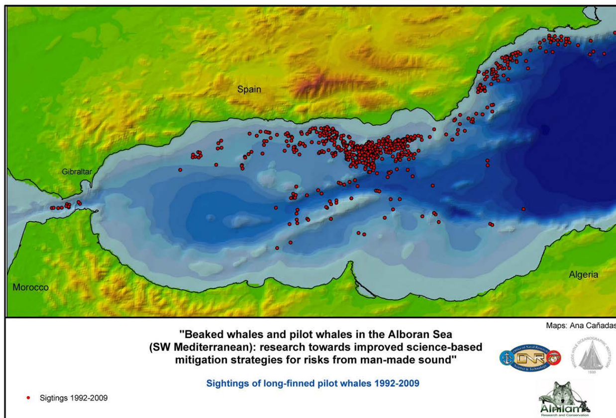
Figure 6. Sightings of long-finned pilot whales from 1992 to 2009 by all ships.
