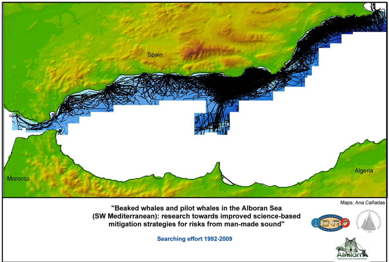
Figure 2. Searching effort from 1992 to 2009 by all ships.
