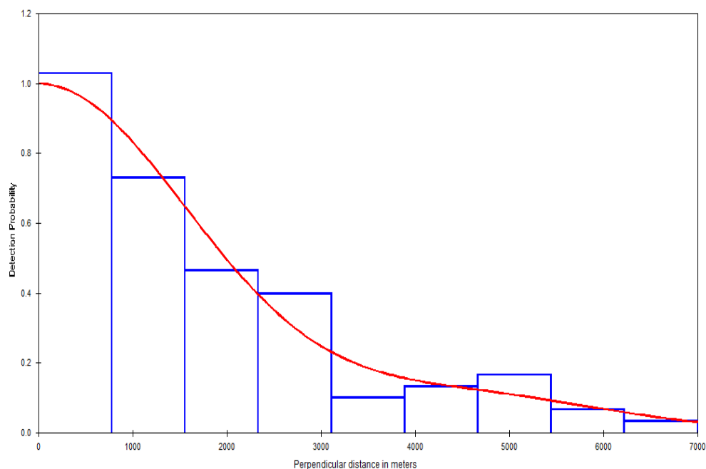
Figure 7. Perpendicular distance distribution (histograms), and fitted detection functions (lines) for the Alliance 2008-2009 dataset for Cuvier's beaked whales.
