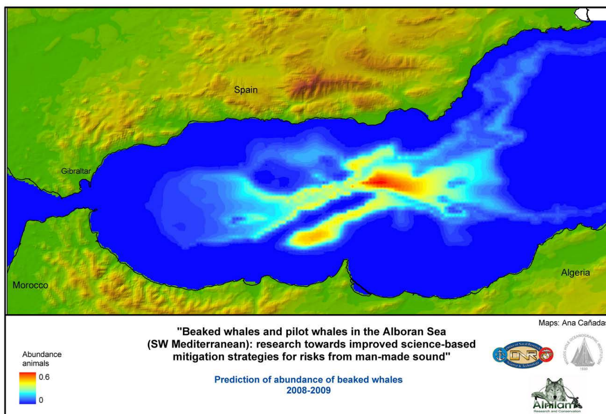
Figure 9. Prediction of abundance of beaked whales for 2008-2009
