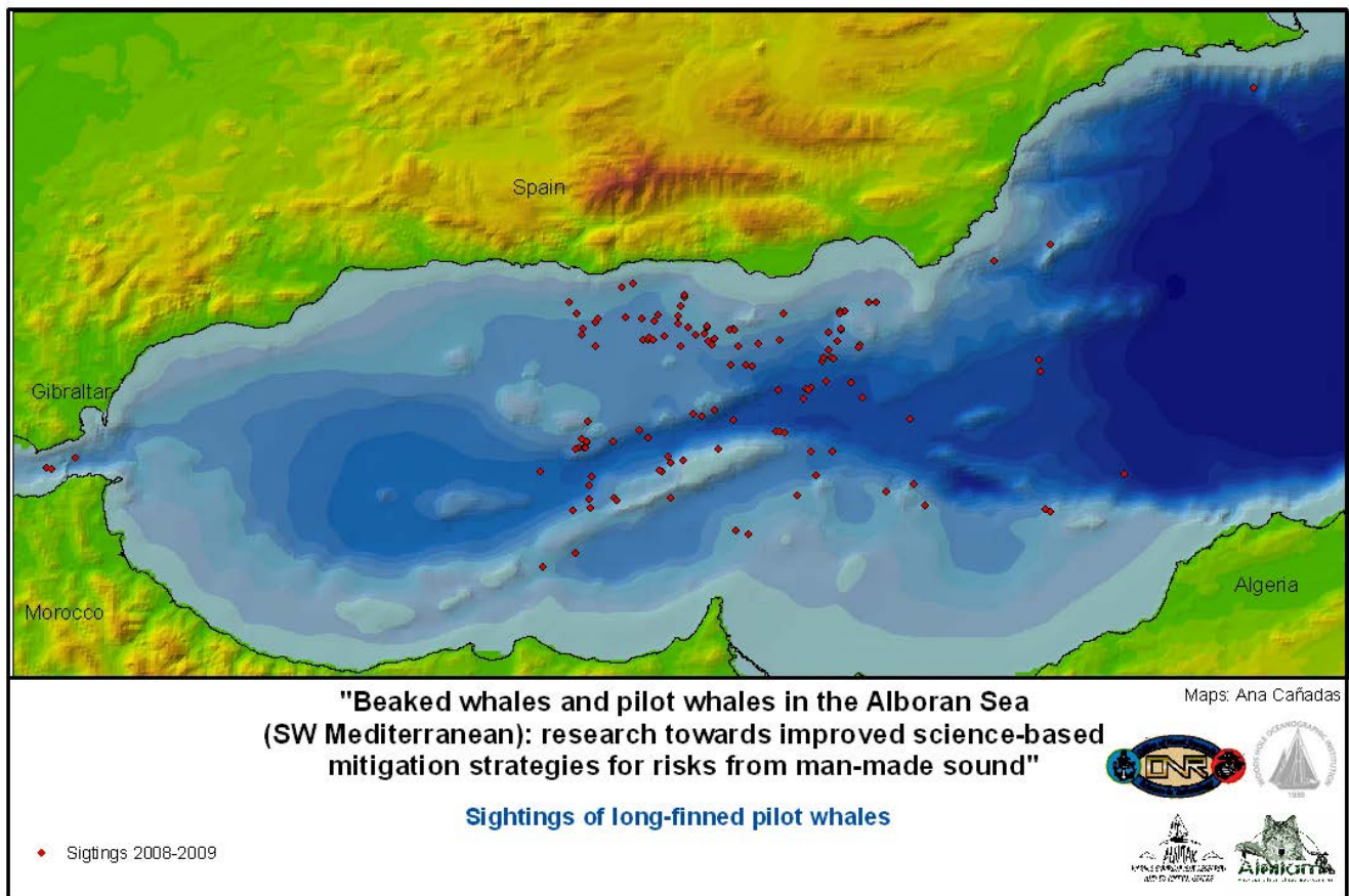
Figure 5. Sightings of long-finned pilot whales in 2008 and 2009 by all ships.
