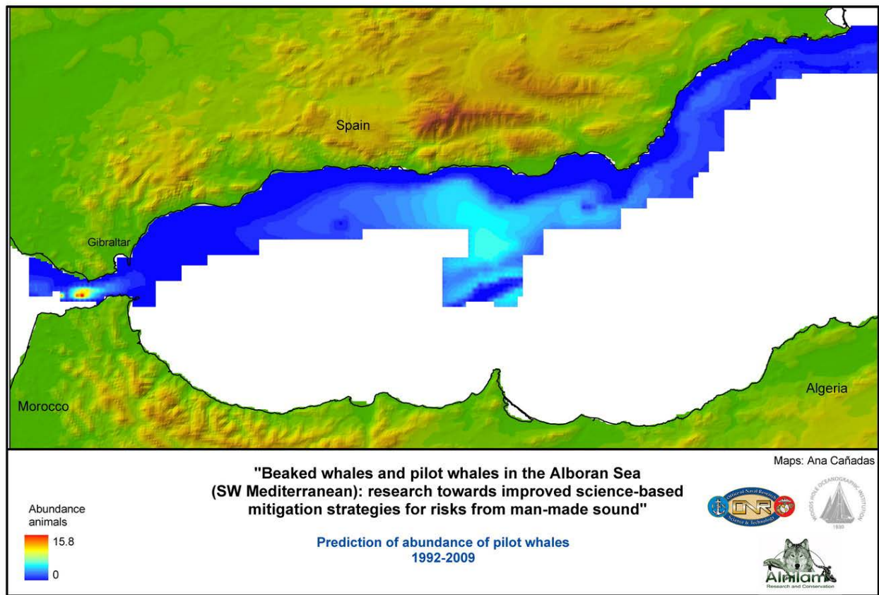
Figure 10. Prediction of abundance of long-finned pilot whale for 1992-2009.
