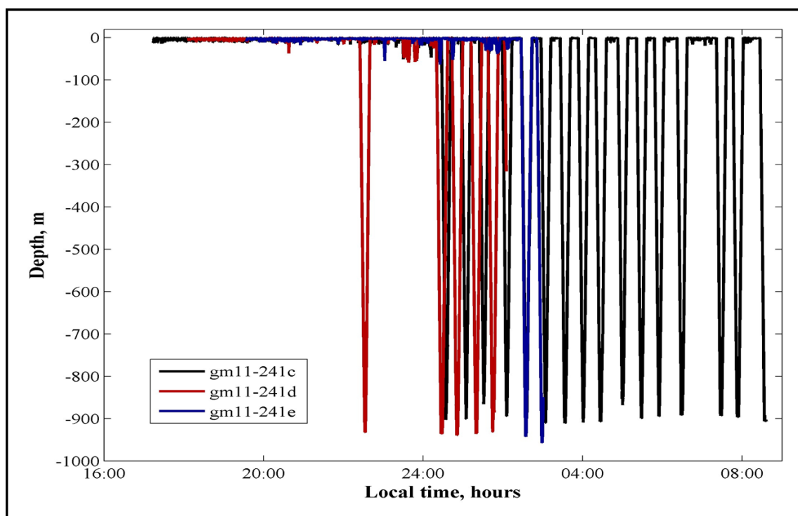
Fig.5. 29-Aug-2011 – Deep overnight dives. Evidence for bottom foraging at >900m of depth
