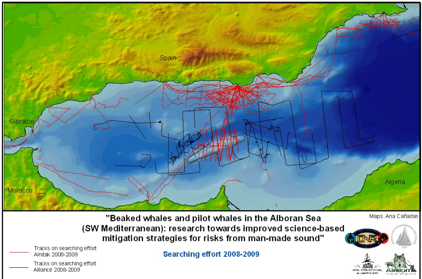
Figure 1. Searching effort in 2008 and 2009 by all ships.
