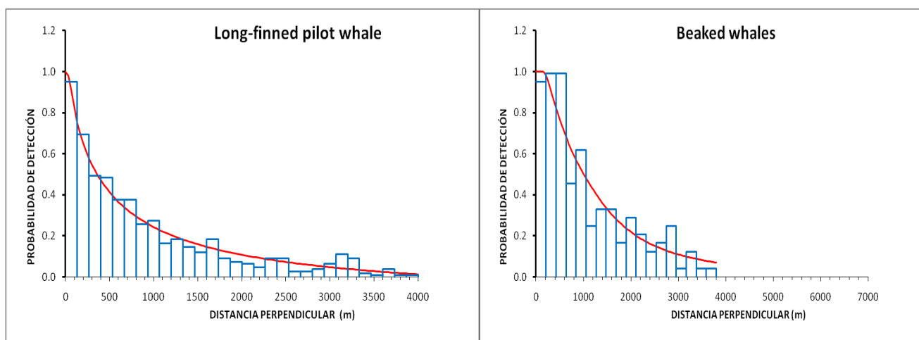
Figure 8. Perpendicular distance distribution, pooled over all covariates (histogram), and fitted detection functions, conditional to the observed covariates (line) for the All ships 1992-2009 dataset.
