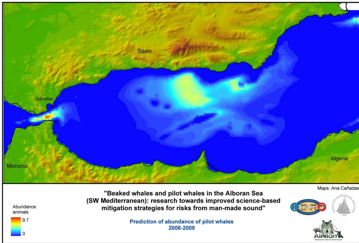
Figure 10. Prediction of abundance of long-finned pilot whale for 2008-2009.
