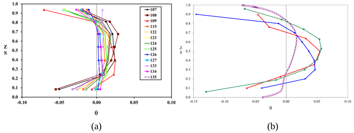
Figure 2.26. a) Combustion simulator generated temperature profiles and b) commercial engine combustor temperature profiles [30].
