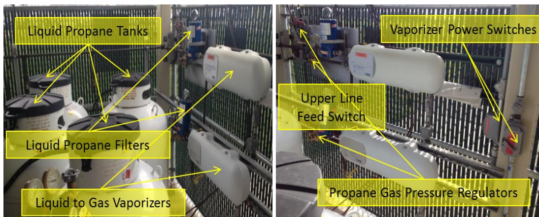
Figure 3.6. Liquid propane to gas propane generation equipment inside AFIT tank barn.
