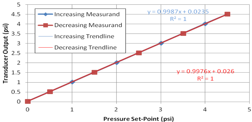
Figure B.2. ESP-32 HD pressure transducer calibration curve
