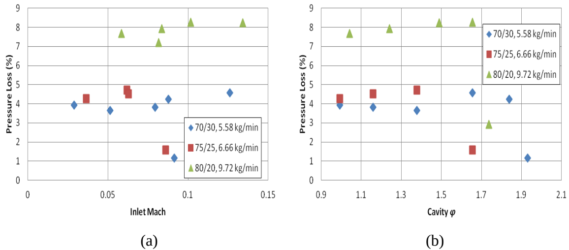
Figure 4.17. Pressure loss as a function of a) exit Mach number and b) cavity equivalence ratio.
