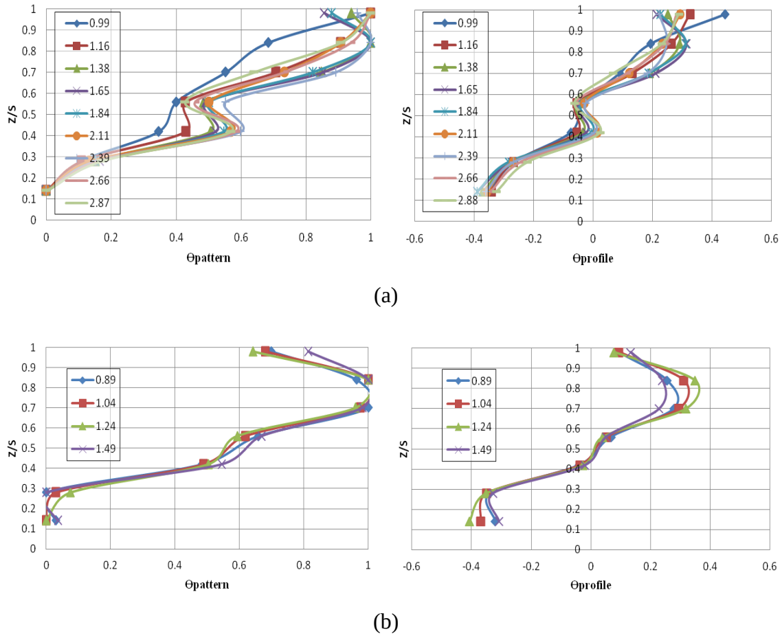
Figure 4.3. Pattern and Profile factors for a) the 75/25 and b) 80/20 flow splits.
