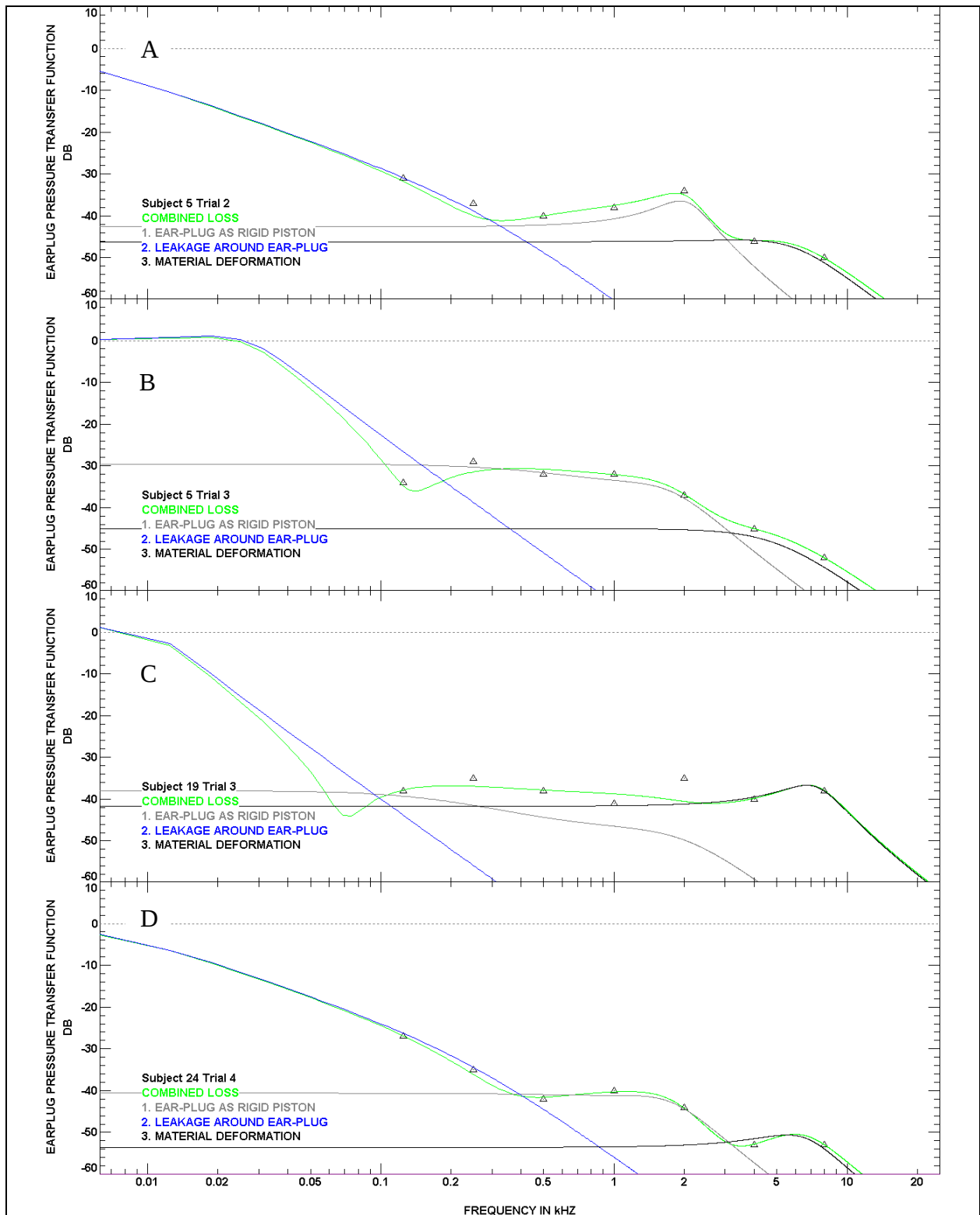
Figure 8. E.A.R. foam earplug. Panel A shows slight leak with low Q, rigid piston with moderately high Q, and SP with low Q. Panel B shows leak with higher Q, causing interference with rigid piston at 125 Hz. Panel C shows lower Q rigid piston with more transmission by SP. Panel D shows three transitions for all three pistons.
