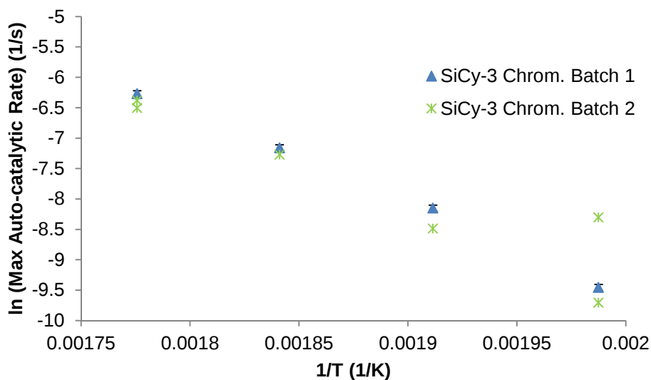
FIGURE S22 Arrhenius plot of two batches of highly purified SiCy-3. The maximum auto-catalytic rate, (d\alpha/dt)_{ac-max} = k_2 \frac{\bar{m}^{\bar{m}} \bar{n}^{\bar{n}}}{(\bar{m} + \bar{n})^{(\bar{m} + \bar{n})}} . This parameter is comparable across samples even when the kinetic parameters differ. In other words, while a higher value of k_2 for a particular sample does not necessarily indicate a characteristically faster reaction if \bar{m} and \bar{n} differ, a higher value of (d\alpha/dt)_{ac-max} always indicates a characteristically faster reaction. Therefore, (d\alpha/dt)_{ac-max} represents the best way to compare the reactivity of samples. The use of auto-catalytic, rather than total, reaction rates, helps to minimize the effect of impurities on the results. Characteristic reaction rates differ by about 10% both between batches, and between multiple samples within the same batch under the same conditions. The calculated activation energies for the two batches differ by about 7%. The analysis also shows that the data below 250 °C (right side of figure) is not highly repeatable, due to the low conversion rates at these temperatures.
