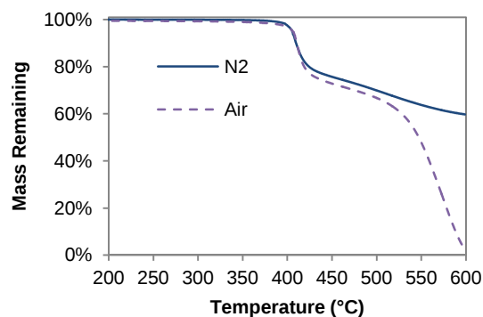
FIGURE S33 TGA traces (in nitrogen and air) of ESR-255 (As-Received) cocured with an equal weight of Primaset® LECy.
