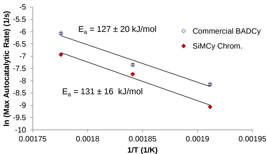
FIGURE S23 Arrhenius plot comparing SiMCy with von t'Hoff purities of 96% (as-synthesized) and >99% (purified via flash chromatography). The highly pure SiMCy reacts at about half the rate of the as-synthesized monomer, while the activation energies do not differ significantly.
