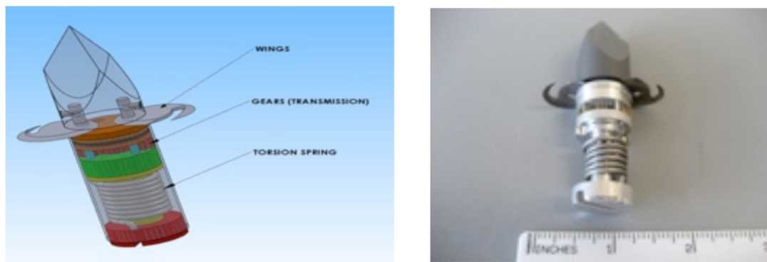
Figure 1. The CAD presentation of the anchoring wing attachment (left image) and the actual prototype without casing (right image). The anchoring wings are shown deployed after a torsion spring via gearing has swung the metal wings perpendicular to the pointed tag tip. The anchoring wing tip would be screwed to the anterior end of an implantable tag.
