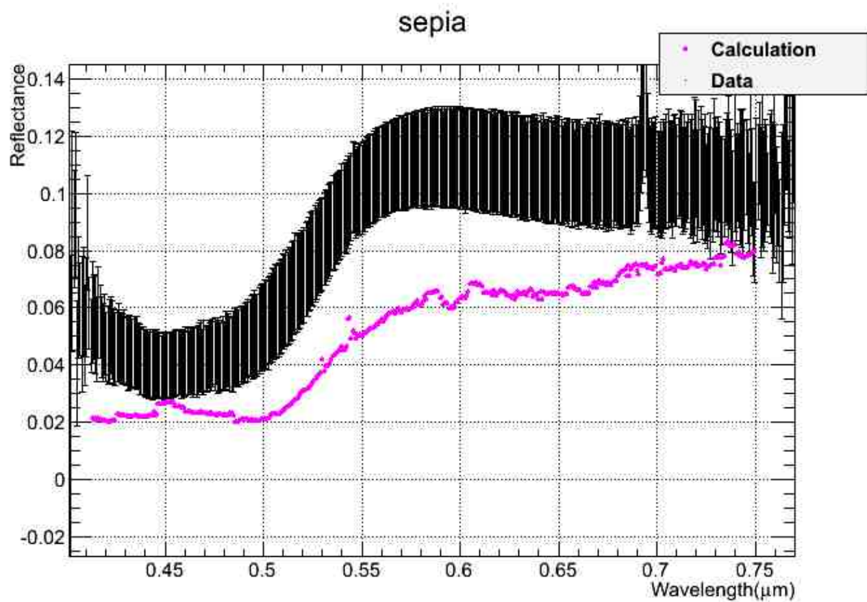
Fig. 10 Reflectance.
