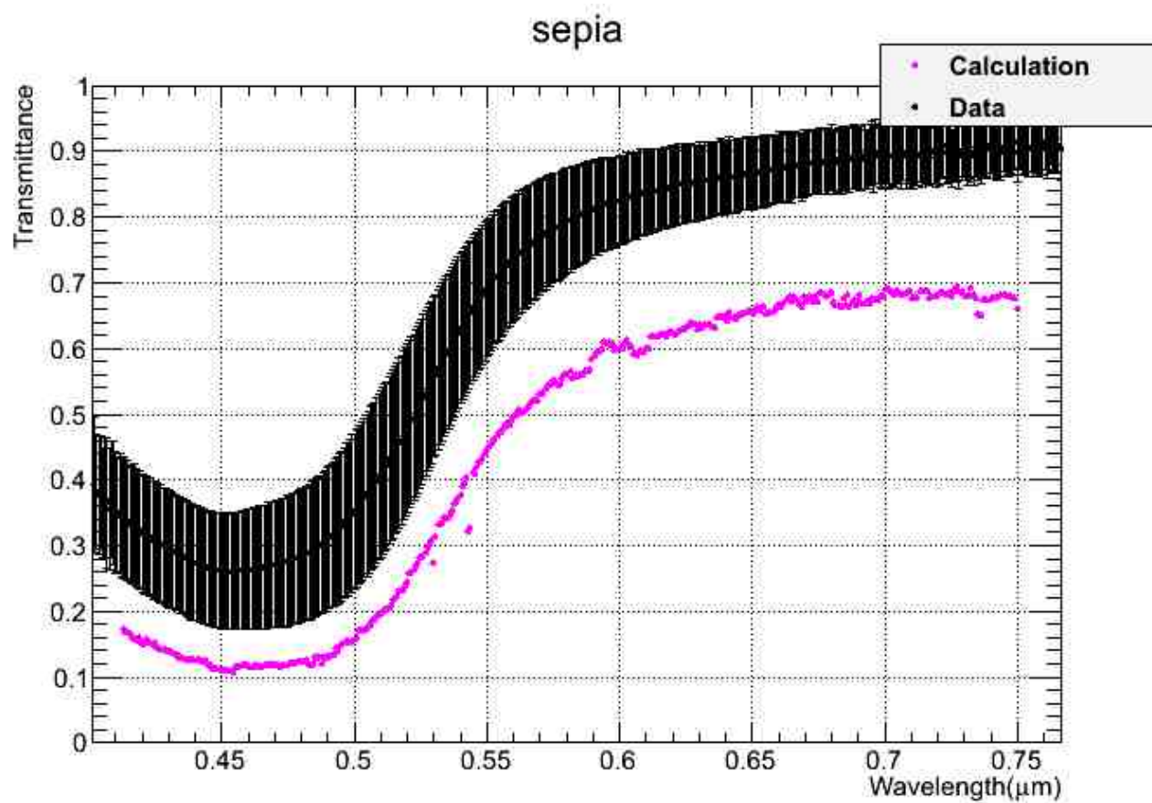
Fig. 11 Transmittance
