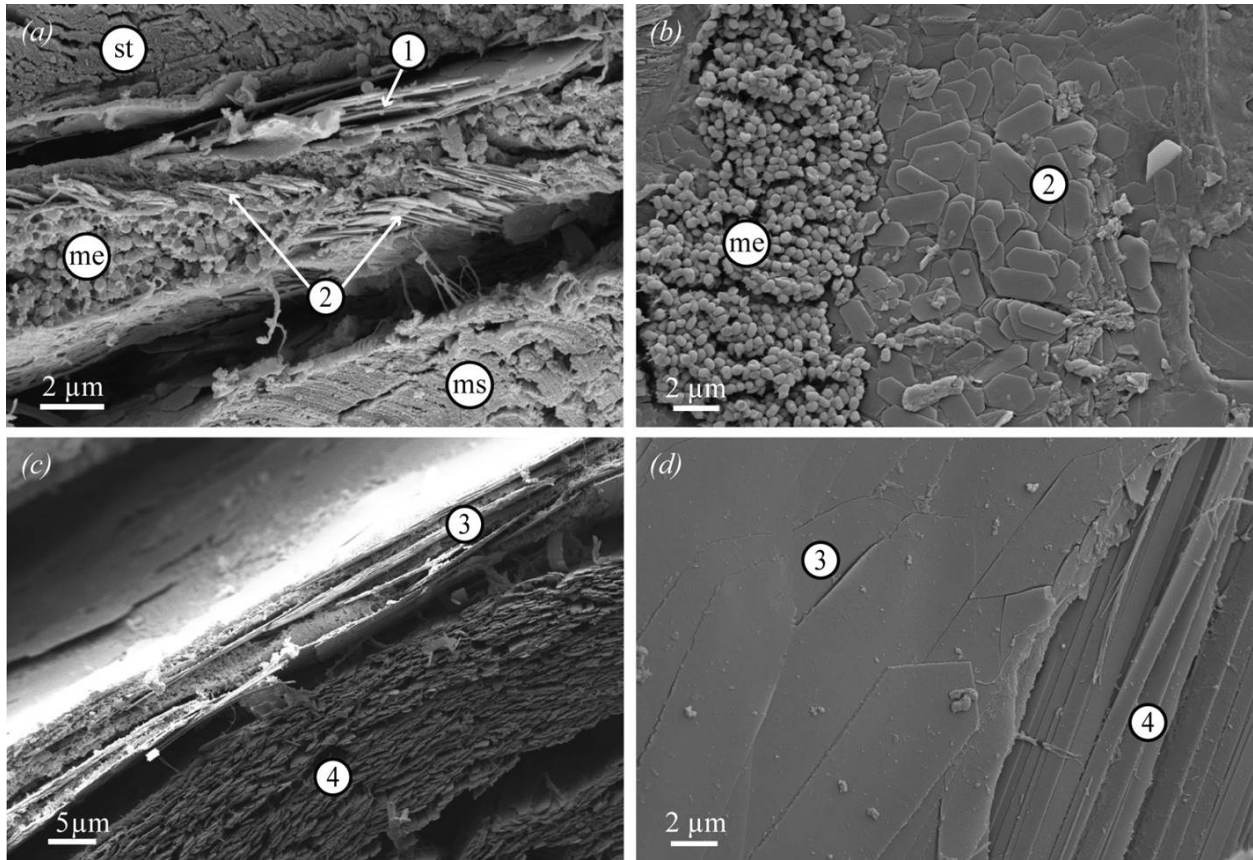
Figure 23. SEM images of the lockdown skin sections from the dorsolateral (a,b) and mid-lateral (c, d) flanks. (a) A cross-section shows Type 1 and Type 2 guanine platelets, melanosomes (me), stratum compactum (st), and muscle (ms) in the dorsolateral flank. (b) A parasagittal section of the dorsolateral skin shows melanosomes and Type 2 guanine platelets with various orientations. (c) A cross-section of the mid-lateral flank shows Type 3 and Type 4 guanine platelets. (d) A parasagittal section of the mid-lateral skin shows Type 3 and Type 4 guanine platelets.
