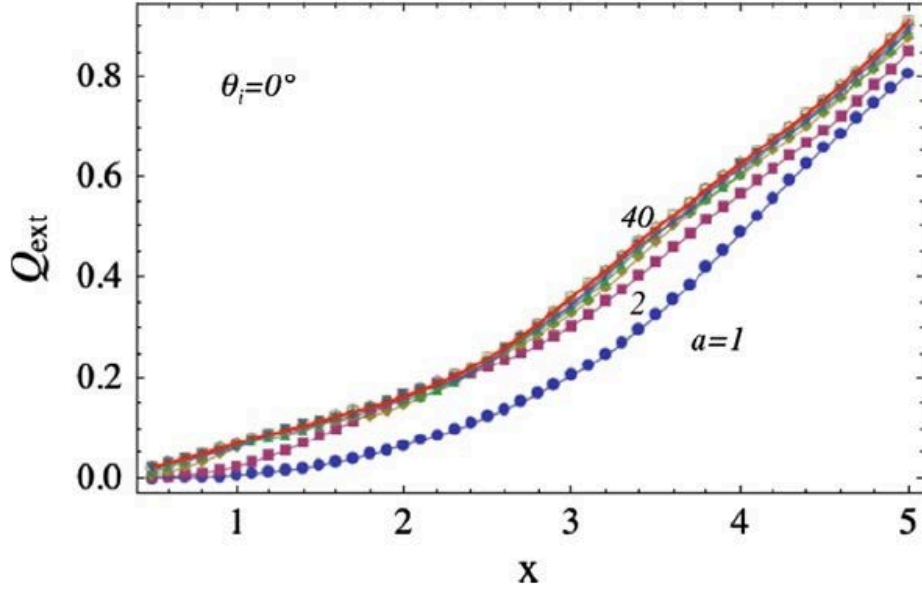
Fig. 1. Extinction efficiency Q_{\text{ext}} versus size parameter x with different aspect ratios: a=1, 2, 4, 6, 8, 10, 20 , and 40 at incident angle \theta_i=0 . The extinction efficiency results for a=4, 6, 8, 10, 20 , and 40 almost overlap each other. The solid red line is the infinite-radius plate results at normal incidence.
