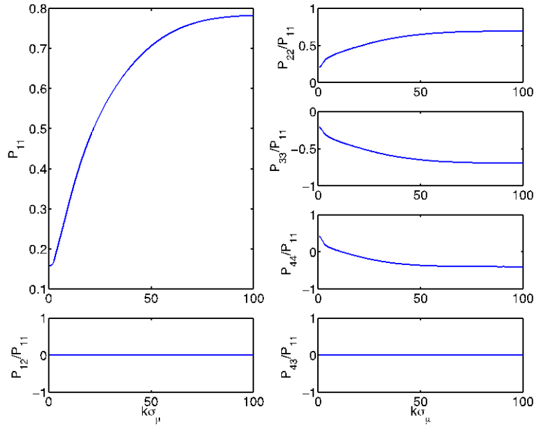
Fig. 7. Mueller matrix elements for a hexagonal ice crystal in the backward direction ( 180^\circ ). The coherence length parameter k\sigma_\mu is from 0 to 100. The hexagonal ice crystal has size parameter kL = 2ka = 150 , where L is the height and a is the semi-width, and refractive index n = 1.31 .
