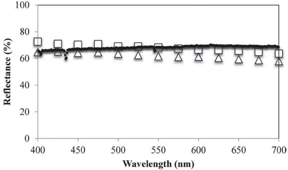
Fig. 2. Simulations show that the cuttlefish fin spot system approximates a Lambertian surface. Dots: Measured reflectance (from 400–700 nm) from cuttlefish fin spot can be as high as ca. 70%, reflecting equally well across the visible spectrum. Triangles: modeled flux reflectance spectrum averaged over all reflection angles and for 0 degree incidence. Squares: the normalized reflectance spectrum obtained by normalizing the modeled reflectance to a perfect Lambertian reflector at the same 0 degree incident and reflection angle, which is commensurate with the measurement. The normalized reflectance averaged over the visible spectrum is chosen to be the same as the measurement (both are 68%).
