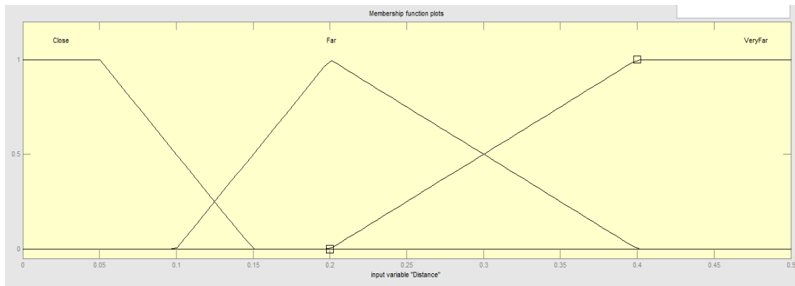
FIGURE 3.5.4: MATLAB 'Distance' membership function schematic.
