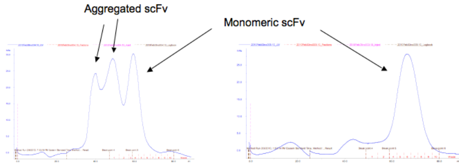
Figure 11. Gel filtration analysis of 8G8F5/2ZCL and ATN-615 scFv
