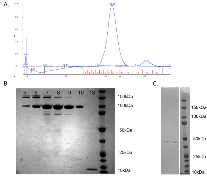
Figure 15. Generation of hu4D5 Fab' for testing the impact of distance on biosensor function. A) Chromatograph of Fab' 2 after pepsin digestion of hu4D5. B) SDS-PAGE analysis of column fractions from "A". C) Native PAGE after reducing fraction 10 to Fab'
