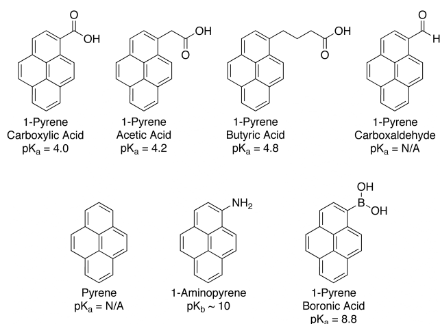
Figure 7. Left: Pyrene compounds utilized to test the importance of the electrostatic interaction for the response mechanism of nanotube biosensors. The pyrene moiety causes these molecules to bind to the nanotube sidewall. The remaining chemical component leads to a known charge (negative, neutral, or positive) at a known location to develop in the nanoscale water layer bound to the surface. Right: Average threshold voltage shift caused by exposure to pyrene compounds. The trend observed is consistent with the expected sign and location of the charge induced in the adsorbed pyrene species. Each value is the average of results from 15-20 devices; error bars are the standard errors of the mean.
