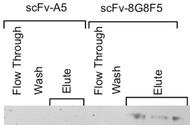
Figure 14. 8G8F5:S=S retains ability to bind PSA
