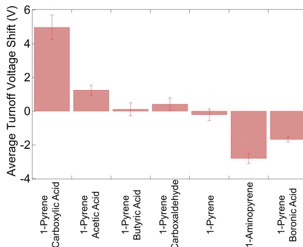
Figure 7. Left: Pyrene compounds utilized to test the importance of the electrostatic interaction for the response mechanism of nanotube biosensors. The pyrene moiety causes these molecules to bind to the nanotube sidewall. The remaining chemical component leads to a known charge (negative, neutral, or positive) at a known location to develop in the nanoscale water layer bound to the surface. Right: Average threshold voltage shift caused by exposure to pyrene compounds. The trend observed is consistent with the expected sign and location of the charge induced in the adsorbed pyrene species. Each value is the average of results from 15-20 devices; error bars are the standard errors of the mean.
