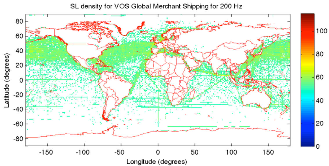
Figure 2. Source level density (dB re (1 microPascal) 2 / Hz @ 1 m/m 2 ) at 200 Hz due to merchant shipping for the year 2004.
