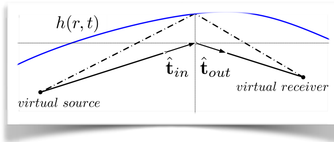
Figure 2: Illustration of how the propagation delay along a surface-reflected eigenray is perturbed due to the surface wave motion.
