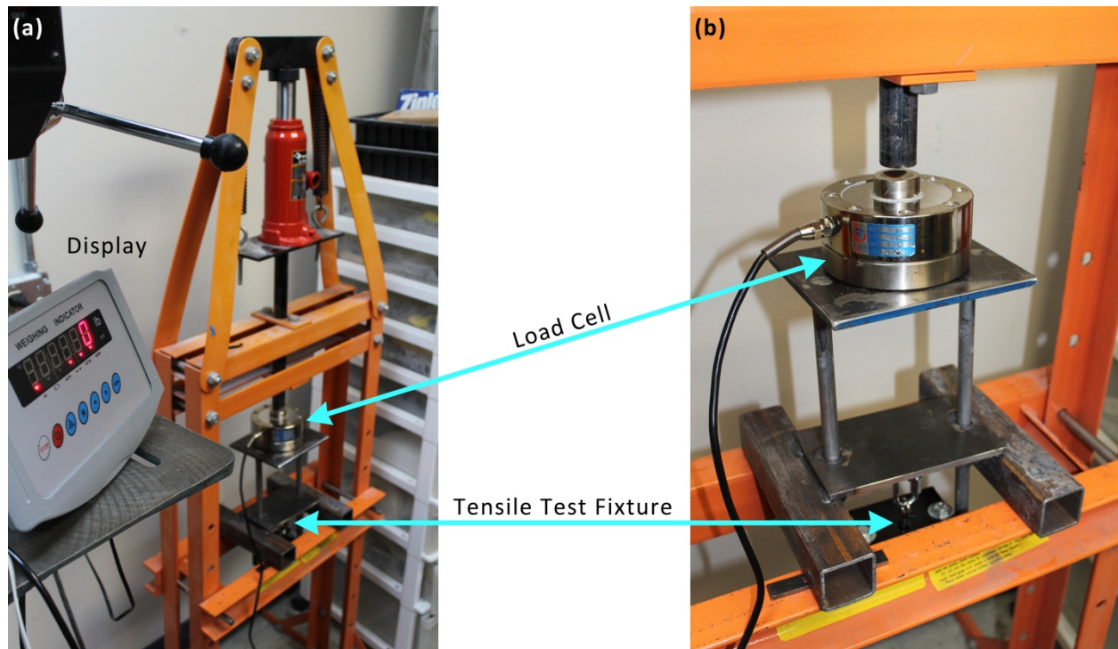
Figure 4: Tensile Test Set-up: showing (1) the fixture and the hydraulic press used to stress the ElectRelease epoxy interface and (2) the load cell and display indicator used to capture the results.
