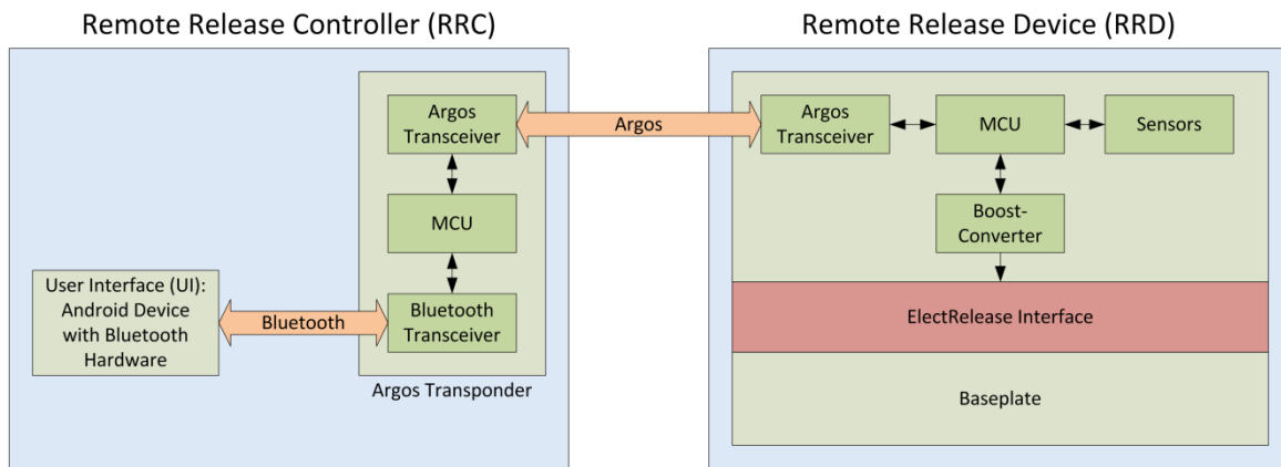
Figure 1: Block diagram of the major system components are highlighted in blue: The RRC is geographically represented “at-the-user” while the RRD is located “on-the-animal.” Long-range communication (< 3.5 km) is accomplished through Argos modulation and depicted by the orange “Argos” arrow. Physically distinct components of these systems are shown in light green: The RRC is comprised of an Android mobile device and an Argos transponder. These components communicate using short-range (< 15 m) Bluetooth modulation that synthesizes a bi-directional serial-data transfer (shown by the orange ‘Bluetooth’ arrow). The RRD is comprised of a baseplate (secured to the study animal) and a reusable platform (that includes its internal electronics and carries a payload). A release mechanism uses ElectRelease epoxy to hold these components together when in deployment mode. When requested to release from the baseplate (release mode), the ElectRelease interface is broken down and the reusable platform is separated from its baseplate. The sub-systems of these components are highlighted in dark green. Both the RRC’s transponder and the RRD’s platform utilize Argos transceivers under autonomous control of microcontrollers (MCUs) running embedded algorithms.
