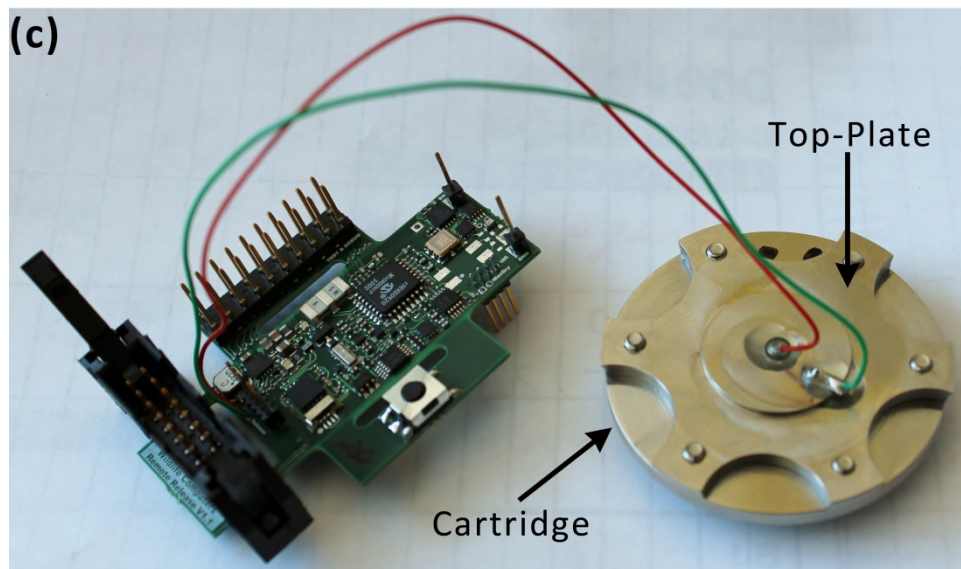
Figure 3: The release mechanism is shown in its various phases of assembly: (a) Bonded Central Structure, (b) Assembled Replaceable Cartridge, and (c) Interfaced with the Electronics.
