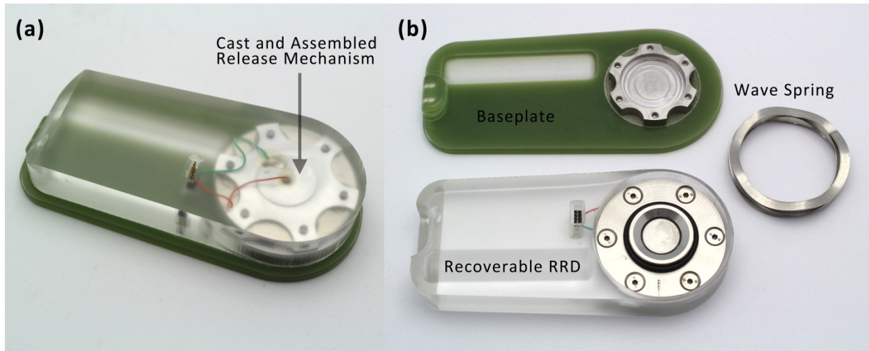
Figure 5: Cast parts of the RRD (omitting circuitry for simplicity) are shown in their (a) fully-assembled or deployed state and (b) in their separated or released state. Note that the base of the release mechanism, the wave spring, and the baseplate will be lost when the RRD is released.
