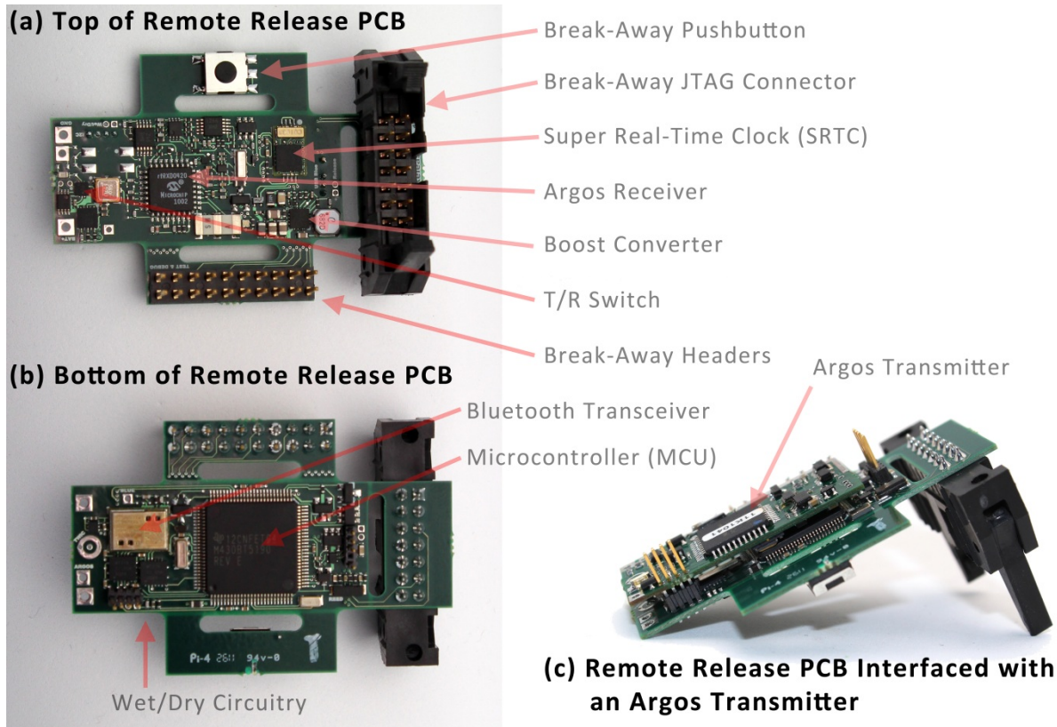
Figure 2: For test and development, the common controller PCBs for both the RRD and the Argos transponder were populated with all components. Additional break-away portions of the board allowed for debugging the functionality of the embedded code. The top (a) and bottom (b) of the control PCB are annotated with their respective components while (c) shows how the design is interfaced with the Argos transmitter.
