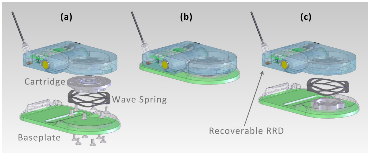
Figure 7: A computer model of the RRD's major components is shown being (a) assembled, (b) deployed, and (c) retrieved.
