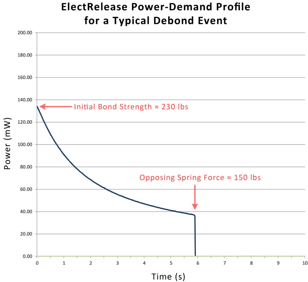
Figure 6: Because it is driven by a constant voltage source, the resistance of the ElectRelease epoxy is shown to monotonically increase as the bond strength is electrochemically degraded. This plot shows the bond strength of the epoxy to weaken to the opposing spring force within 6 seconds of being actuated. At which point the bond fails and the device is released.
