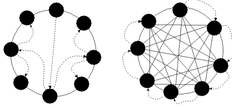
Figure 8: Simple-cycle and fully connected blocks
