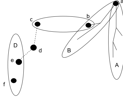
Figure 7: Limited-block example. Ellipses denote blocks, solid circles - agents, solid lines - ordering relationships, dotted lines - edges of the constraint graph
