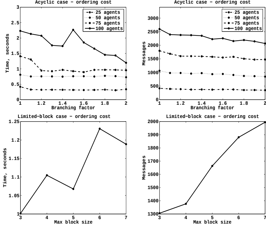
Figure 9: Ordering costs for acyclic (top row) and limited-block (bottom row) cases
