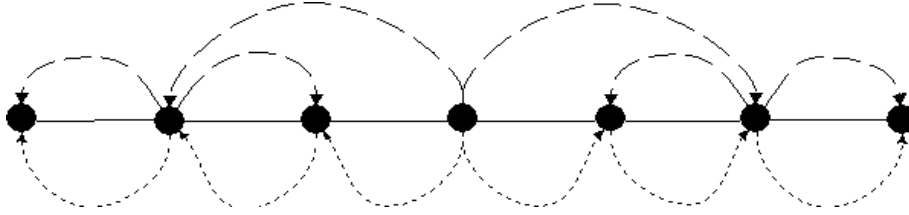
Figure 1: 7-nodes chain constraint graph. Dotted arrows mark DFS tree ordering. Dashed arrows - pseudo-tree ordering.
