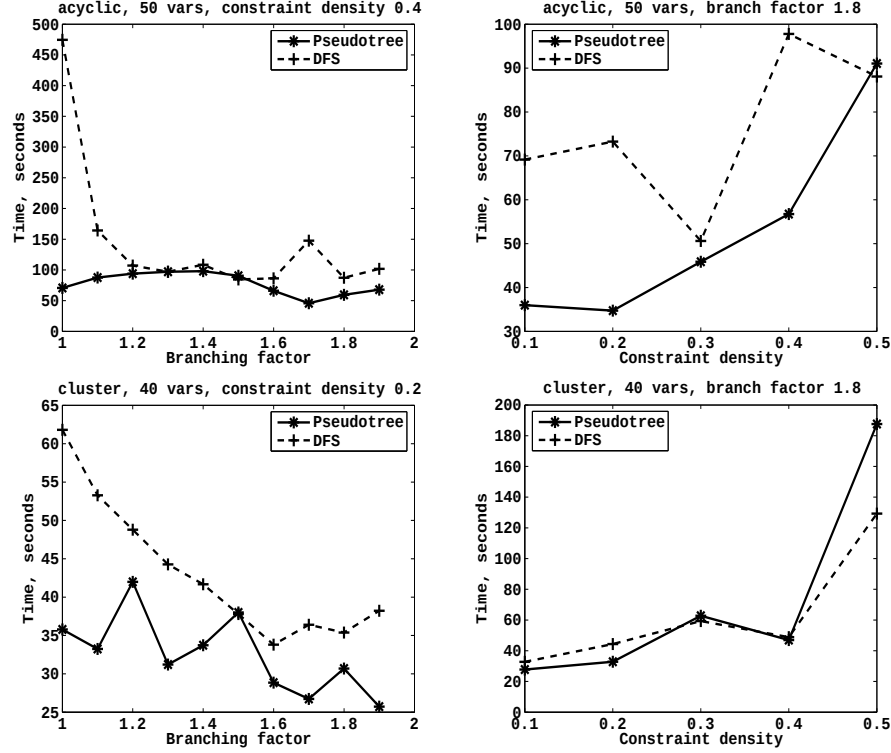
Figure 10: ADOPT performance using DFS and pseudotree orderings. Acyclic constraint graphs (top row) and limited-block case (bottom row)
