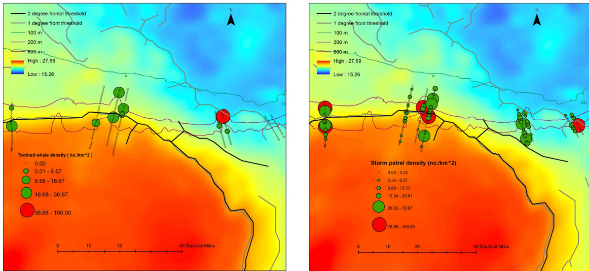
Figure 4 – Distribution of odontocetes (left panel) and storm petrels (right) observed during the 2010 R/V Connecticut shelfbreak survey plotted relative to satellite observations of sea surface temperature and derived estimates of the location of temperature fronts
