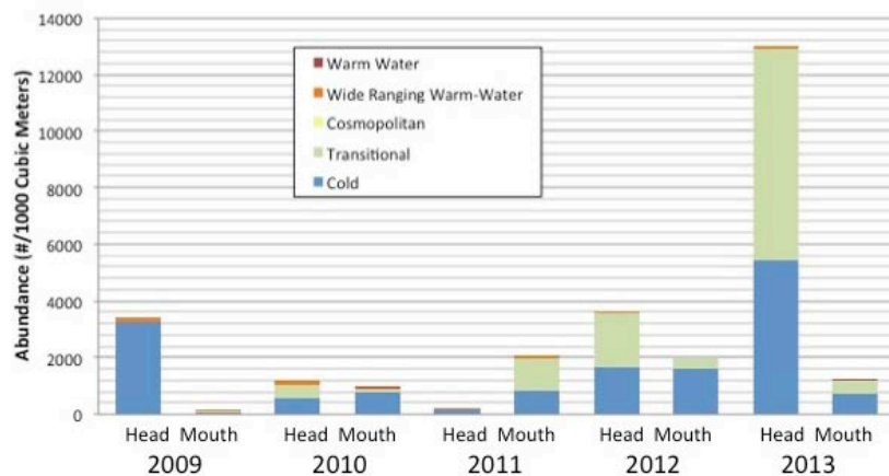
Figure 3 – Euphausiid abundance grouped by watermass type from SEA net tows targeting the head and mouth of Atlantis Canyon in 2009-2013
