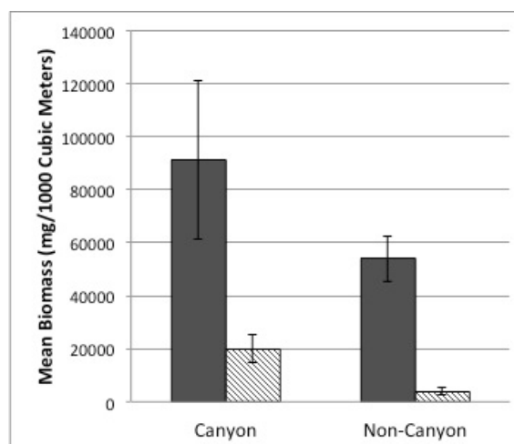
Figure 2 – Mean euphausiid biomass sampled at canyon heads (dark grey) and mouths (light hatched grey) and at locations of comparable shallow (dark grey) and deep (light hatched grey) depths at sites away from canyons
