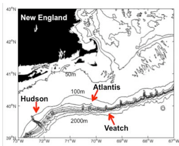
Figure 1 – Canyons of the New England shelf break. Arrows show the three canyons studied here, for which data are available.
