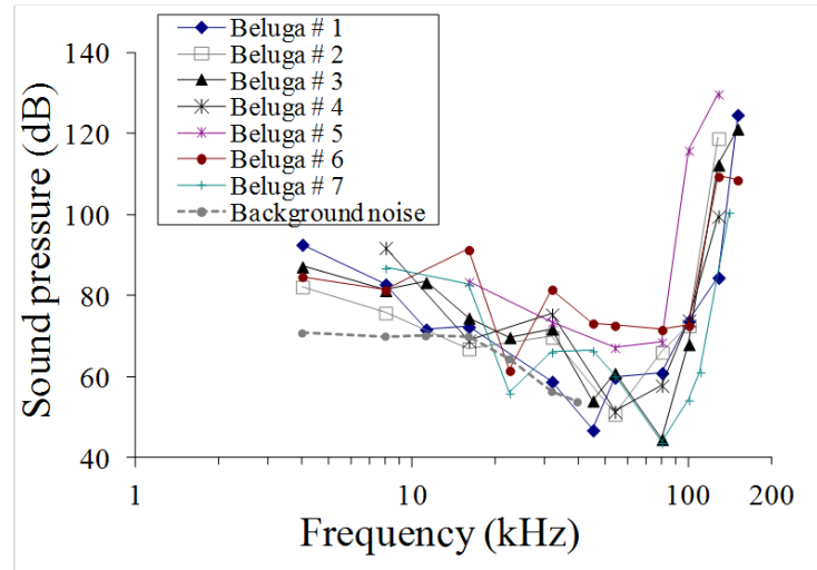
Figure 2. AEP audiograms of all seven wild belugas and Bristol Bay background noise spectrum. Sound pressure levels are in dB re 1 \mu Pa.
