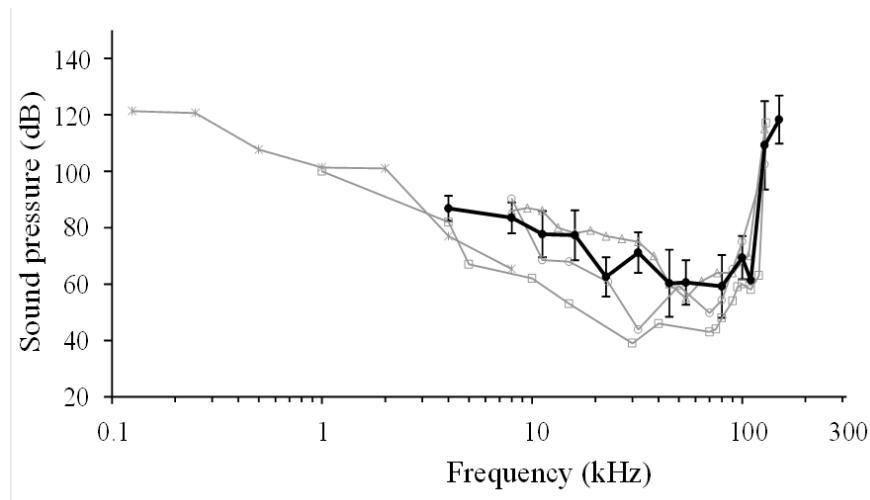
Figure 4. Mean wild beluga audigram \pm s.d. (black, circles) compared to the audigrams (grey and/or open symbols) from belugas held in laboratory conditions or in aquaria. Other audigrams include: (White et al., 1978)-squares, (Awbrey et al., 1988)-stars, -circles, (Klishin et al., 2000)-triangles, (Finneran et al., 2005)-x's, (Ridgway et al. 2001)-dashes. The audigram (x shapes) which cuts off near 50 kHz was considered a result of aminoglycoside antibiotic treatment. All other audigrams are similar to the wild belugas. Sound pressure levels are in dB re 1 \mu Pa.
