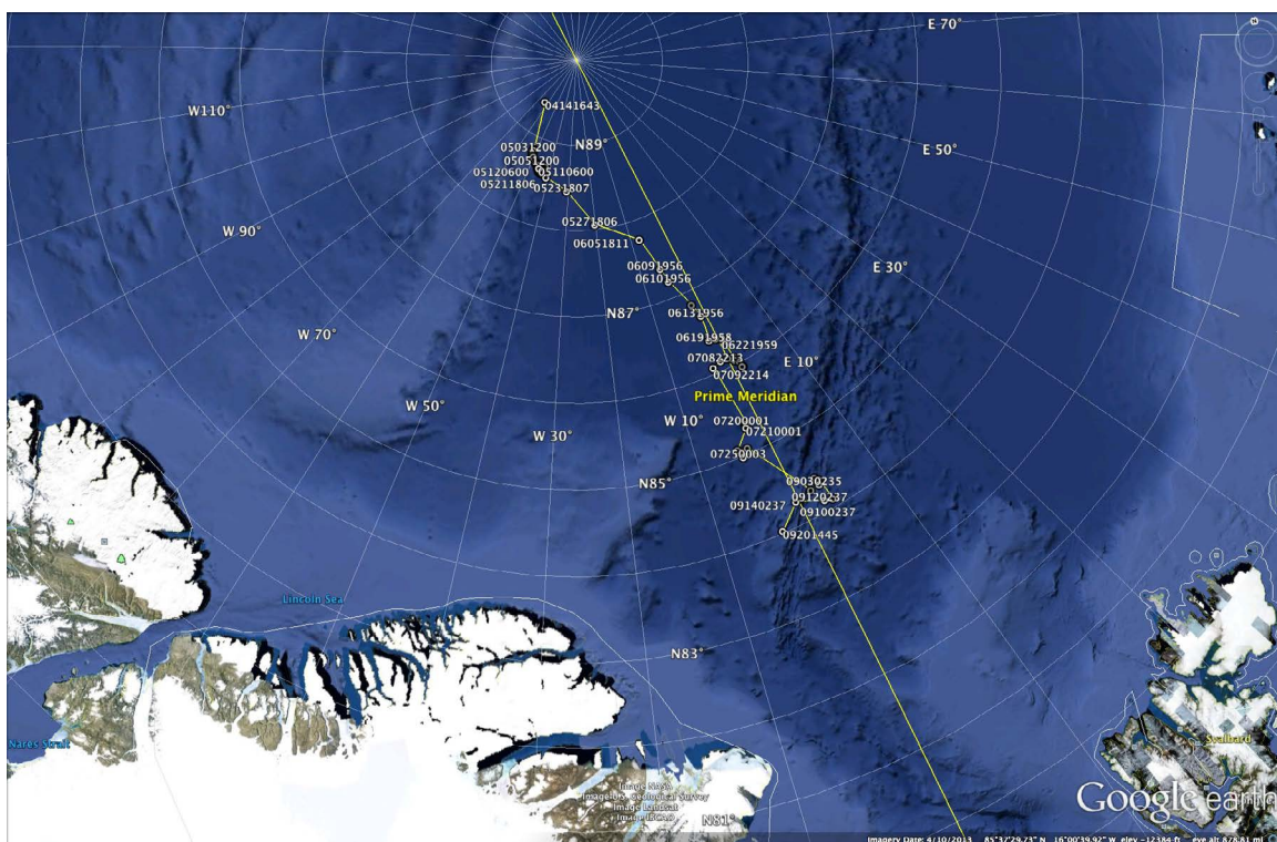
Fig. 3. Drift of the SIO-WHOI THAAW mooring showing the track from deployment at ice camp Barneo on 14 April 2013 until it was sighted on the surface by the KV Svalbard on 20 September 2013. A subset of the GPS positions provided by the GPS-Iridium beacon are labeled in mmddhhmm format.
