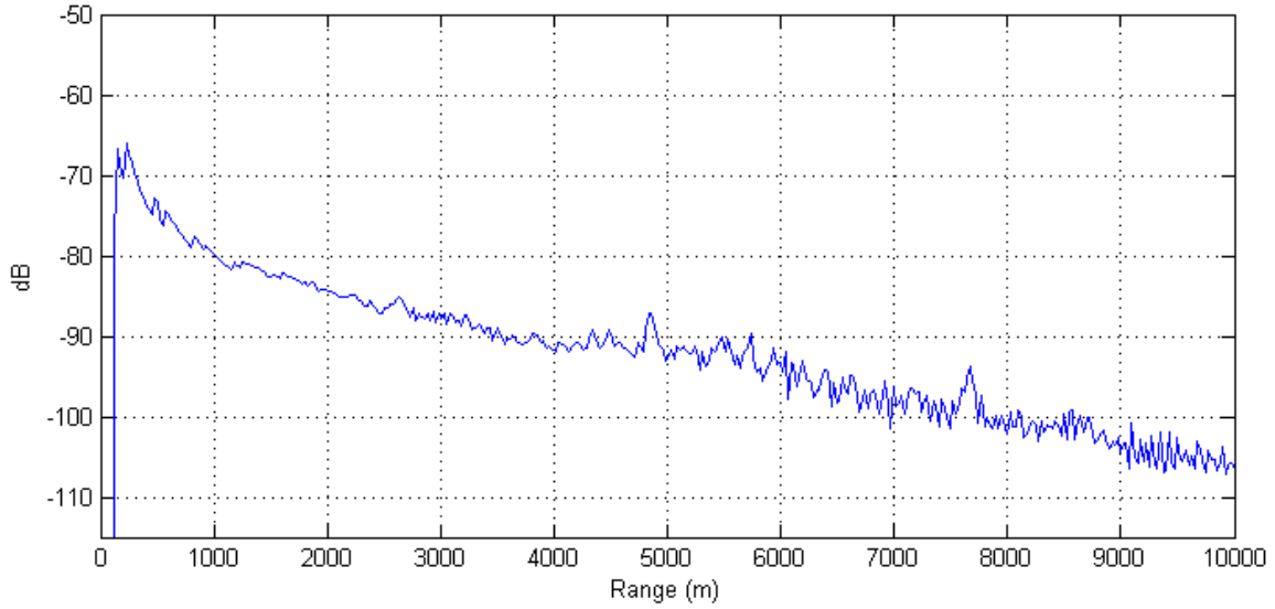
Fig. 5(c): Ridge with fixed SSP ('V'-shaped refracting duct) – bottom reverberation
