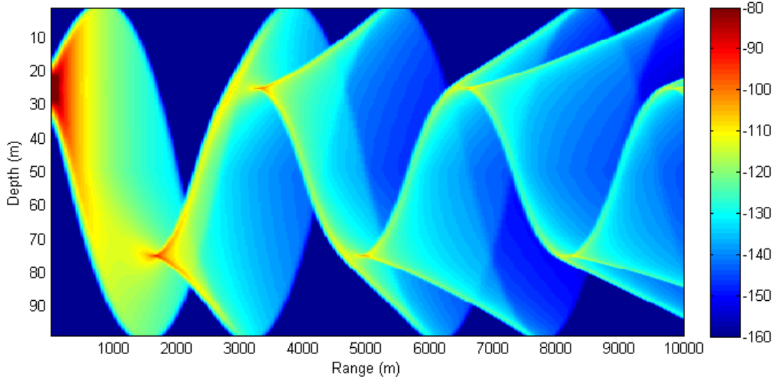
Fig. 2: Range-independent refracting duct
