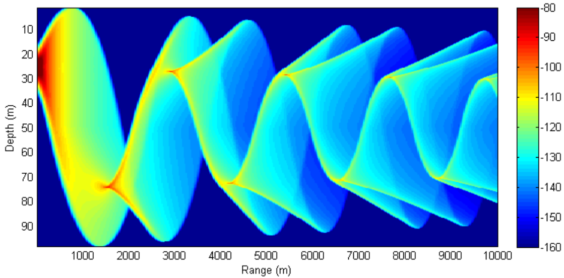
Fig. 6: Fixed water depth with varying SSP
