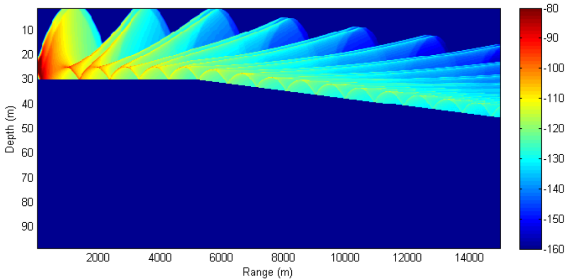
Fig. 3(a): Downslope with downward refraction – waterborne paths alone
