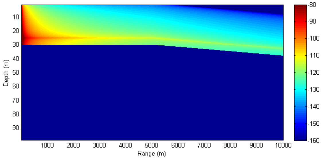
Fig. 3(c): Downslope with downward refraction – flux
