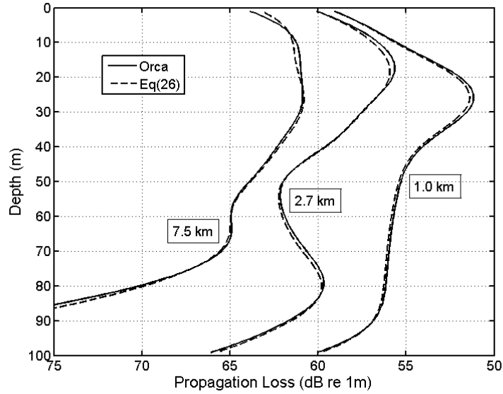
Fig. 1: Comparison with Orca of range-averaged propagation loss vs depth at selected ranges in an upward refracting stratified environment [taken from Fig 6 of Harrison(2013)].
