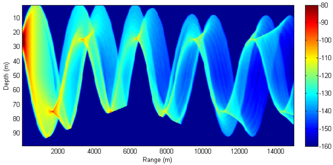
Fig. 5(a): Ridge with fixed SSP ('V'-shaped refracting duct) – waterborne paths
