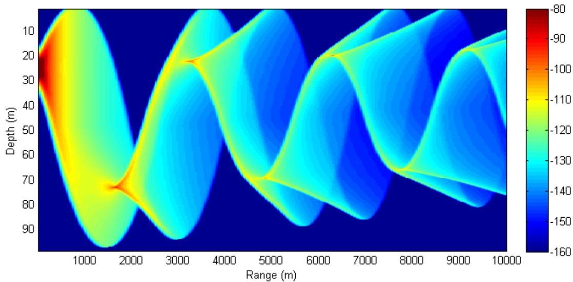
Fig. 7: SSP squeezed to varying water depth
