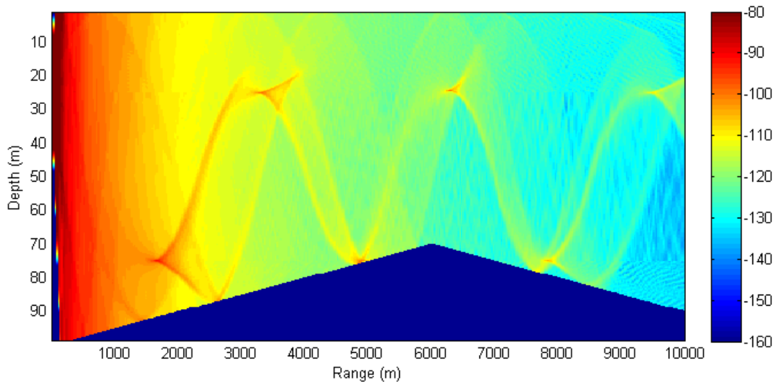
Fig. 5(b): Ridge with fixed SSP ('V'-shaped refracting duct) – all paths
