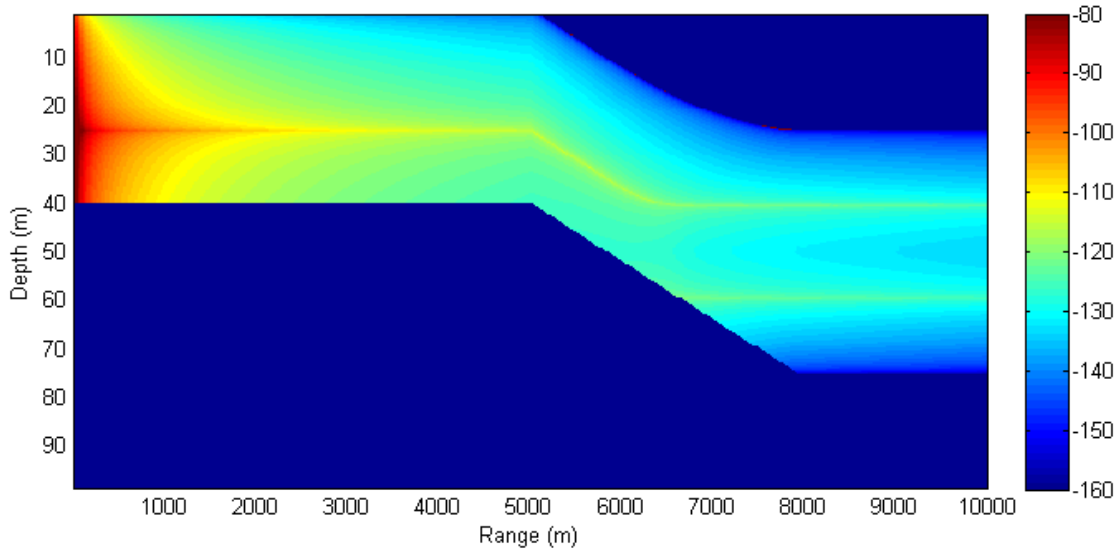
Fig. 4(d): Downslope with fixed SSP ('V'-shaped refracting duct) – flux
