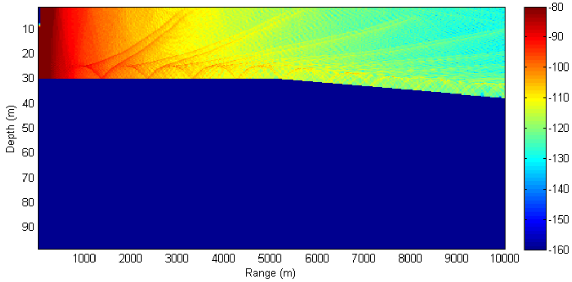
Fig. 3(b): Downslope with downward refraction –all paths
