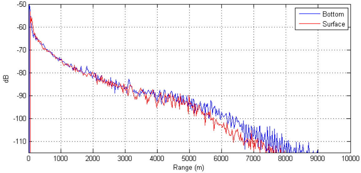
Fig. 4(c): Downslope with fixed SSP ('V'-shaped refracting duct) – bottom reverberation (blue), surface reverberation (red)
