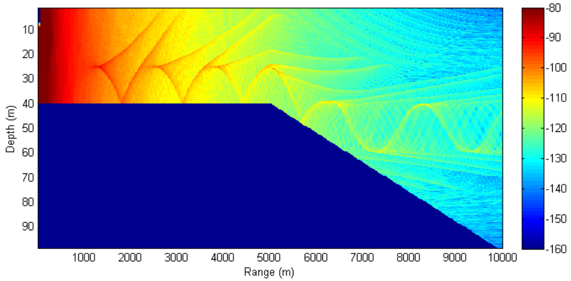
Fig. 4(b): Downslope with fixed SSP ('V'-shaped refracting duct) – all paths
