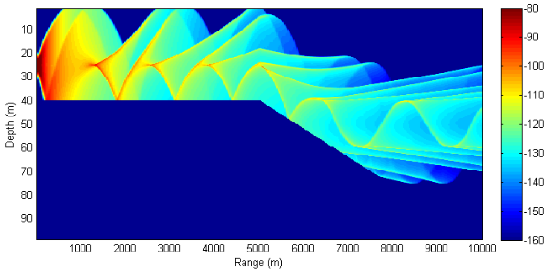
Fig. 4(a): Downslope with fixed SSP ('V'-shaped refracting duct) – waterborne paths
