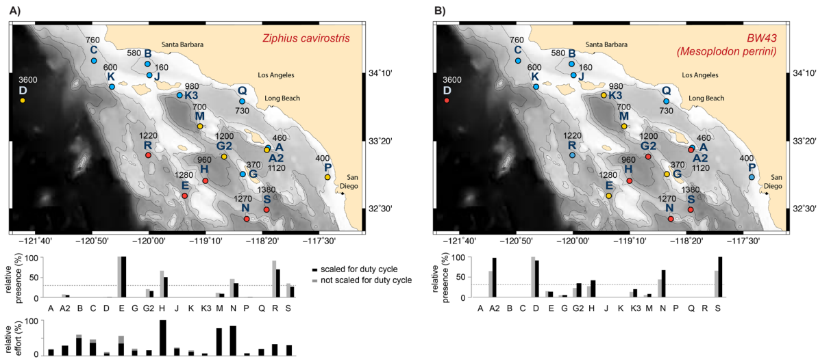
Figure 2: Distribution map of A) Ziphius cavirostris (Cuvier's beaked whales) FM pulse and B) BW43 FM pulse detections (likely produced by Mesoplodon perrini , Perrin's beaked whales) across the Southern California Bight (SCB). Site name (letter) with depth (m); sites with strong relative beaked whale presence in red (>33% relative presence), sites with low relative presence in yellow, sites with no detections in blue. Presented are automatically detected and manually verified beaked whale detections from 18 sites and 126 deployments. Histograms at the bottom show relative presence across sites and relative recording effort. Some sites were on a duty cycle during some deployment periods (grey bars). This reduced recording time is being adjusted for (black bars).
