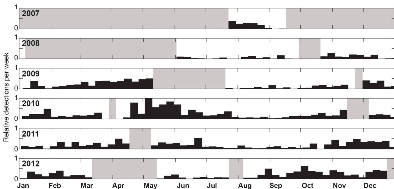
Figure 3: Weekly relative Cuvier's beaked whale FM pulse detections from 2007 until 2012 at site H. There appears to be a seasonal component to the presence of beaked whales at this site with generally lower probability of detection during summer and early fall months.
