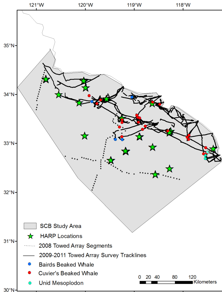
Figure 1: SCB towed array data (black tracklines) from the years 2008-2011 with detections of Baird's (blue), Cuvier's (red), and unidentified beaked whales (turquoise). Grey area denotes polygon over which habitat modeling will be performed.
