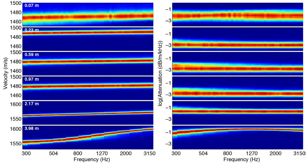
Figure 2 sediment dispersion curves at several depths below the seafloor. The red regions are approximately the 95% confidence interval for the solution.
