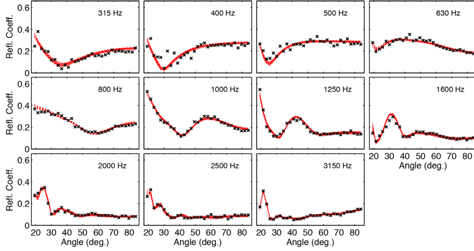
Figure 1 Measured reflection coefficient (x) along with the 95% highest probability distributions inversion fits (lines).
