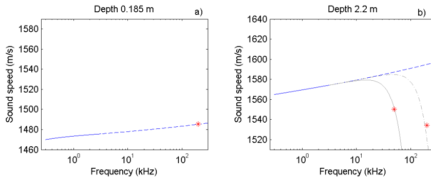
Figure 3. dispersion from inversion of reflection data (solid) compared with core data (*) at depths where a) there were no shells, 0.185 mbsf and b) shells were present 2.2 mbsf. The dashed lines are VGS predicted from the MAP model derived from the reflection data. The core measurements in the shelly layer have been interpreted with a multiple scattering model corresponding to particle sizes of 2 mm (dashed gray) and 6 mm (solid grey).
