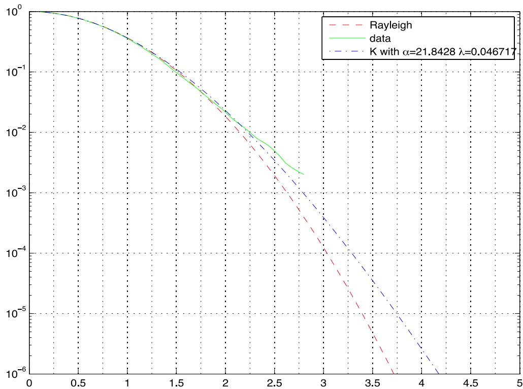
Fig. 1 Plot of beam time series statistics from GULFEX12 for a triplet broadside beam compared to Rayleigh and K-distributed statistics, using a 0.1~s LFM from 2500--3500 Hz.
