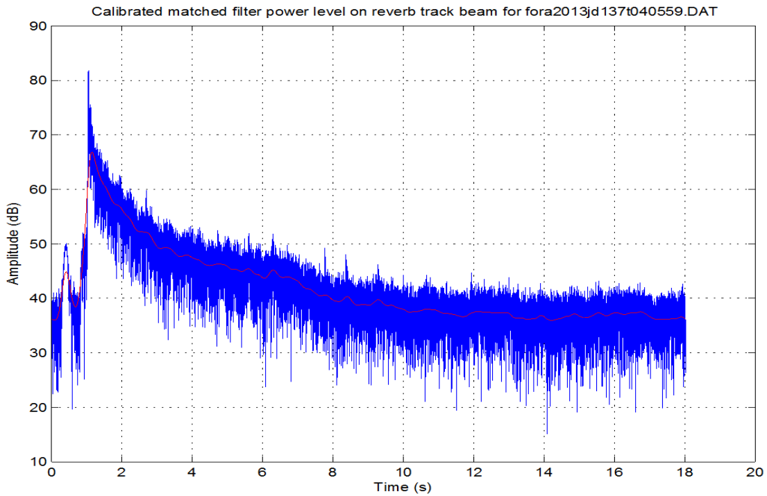
Fig. 3. Sample matched filter output from TREX13 for a 1 s LFM pulse from 1800–2700 Hz for a beam looking along the designated ‘Reverb Track’; bearing 129° T (triplet beamforming). Also shown in red is the Gaussian smoother filter output used to estimate the incoherent reverberation levels which are more useful for modeling comparisons.
