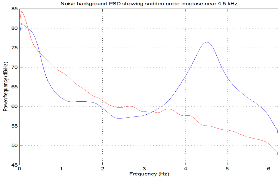
Fig. 2 Noise power plots illustrating a mysterious nighttime noise in the 4 -5 kHz region that was observed nightly during the TREX13 experiment (blue line). The red line shows a typical daytime ambient spectrum.
