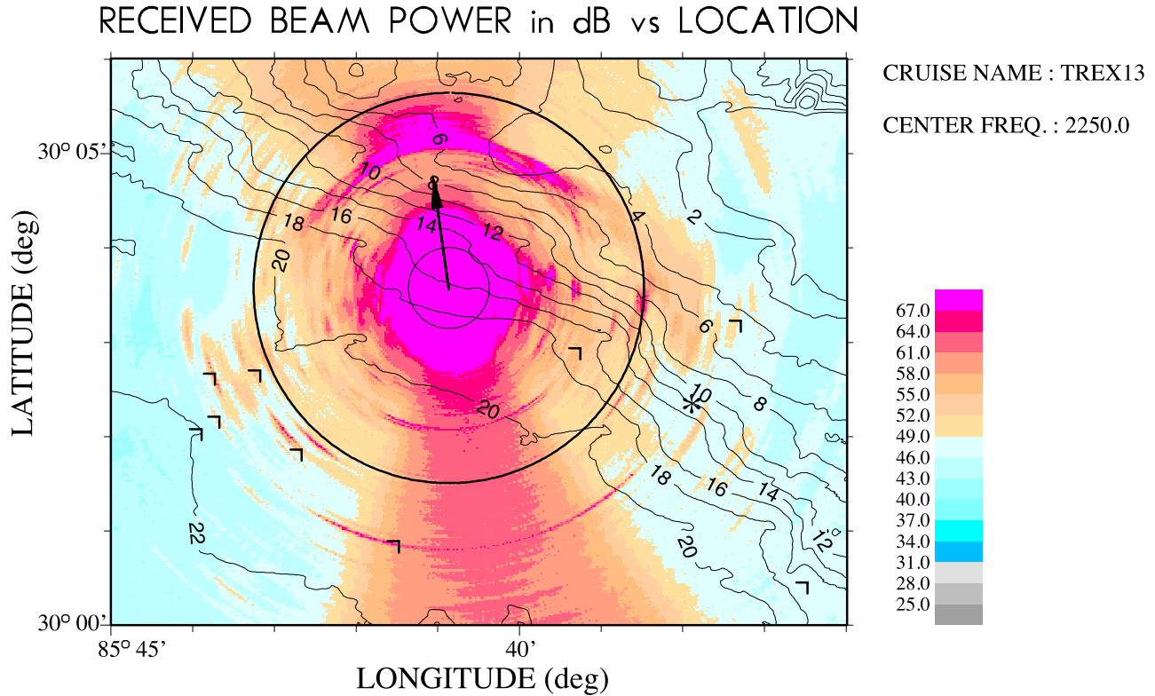
Fig. 4 Polar plot of reverberation vs. location from TREX13 using the FORA off Panama City, FL from a 1 s LFM; 1800–2700 Hz (triplet beamforming). Water depth 18 m; source depth 17 m; receiver depth 16 m. Black angle bracket symbols show the locations of shipwrecks and other man-made sources of clutter.
