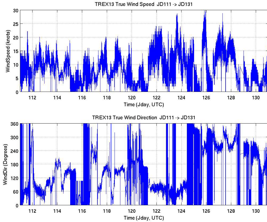
Figure 3. TREX13 wind speed and direction observed by the R/V Walton Smith 22 April – 10 May 2013.
