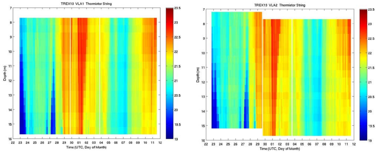
Figure 2. TREX13 water column temperature structure observed 22 April – 12 May 2013. (Left) VLA1 (2.4 km range). (Right) VLA2 (4.2 km range).
