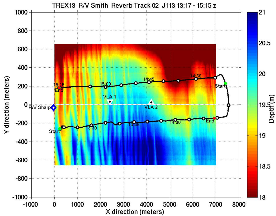
Figure 4. Source tow track Reverb Track 02 along with the Main Reverberation Track bathymetry.
