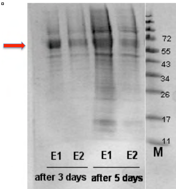
Fig. 2. Small-scale expression of rhAChE. Expression was tested in 293T cells, and the protein was secreted into the medium
