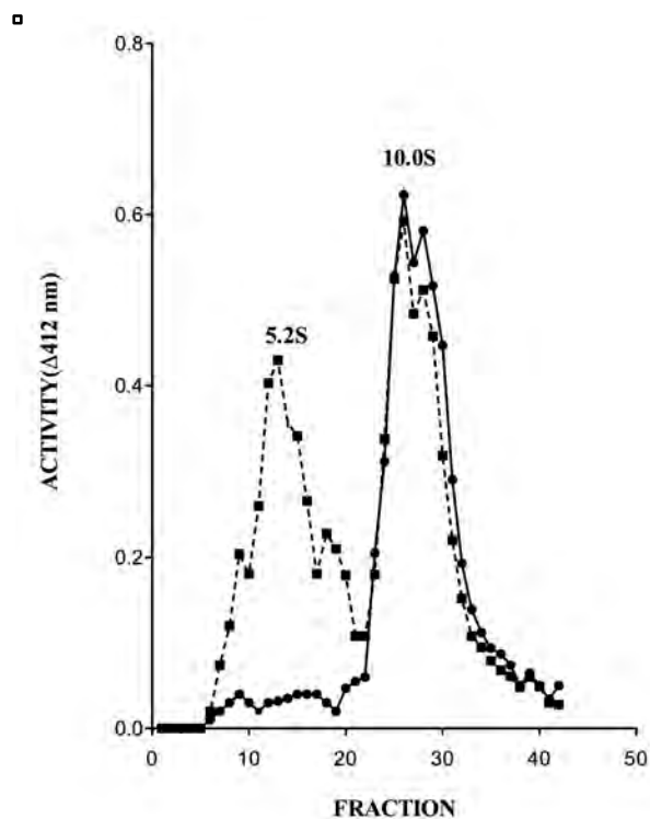
Fig. 10. Sucrose gradient centrifugation of DG-rhAChE T . Centrifugation was on 5-20% sucrose gradients in 1% Triton X100/PBS, pH 7.0. ■---■---■, DG-rhAChE T in the absence of PRAD; ●-●-●, DG-rhAChE T preincubated with PRAD.
