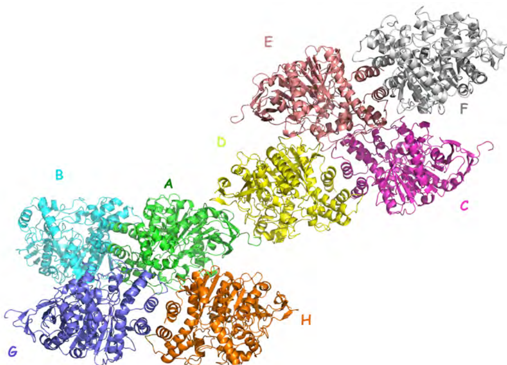
Fig. 14. Symmetry-related molecules in the P2_12_12_1 space group of mAChE (PDB1JO6)
