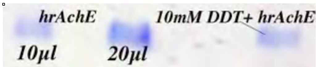
Fig. 3. Non-denaturing PAGE gel for purified rhAChE in the absence (left & center) and presence (right) of DTT.
