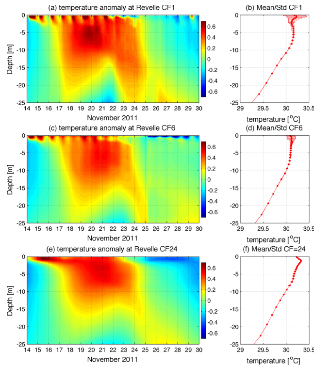
Figure 2. (Left) Time-depth diagrams of the upper ocean temperature [ ^{\circ}\text{C} ] sampled along the Revelle track from (a) CF1, (c) CF6 and (e) CF24. (Right) Mean temperature profiles overlaid with the diurnal standard deviation.
