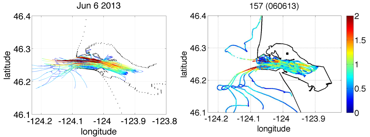
Figure 1. Drifter speed tracks for June 6, 2013 at the Mouth of the Columbia River. The color of the line is the drifter speed. Speed color scale plotted to the right (m/s). Black lines/dots indicate land boundaries. Left panel: Delft3D forecast. Right panel: Observations.
