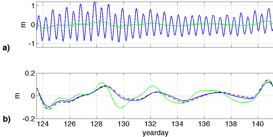
Figure 2. a) Measured ocean sea-surface elevation for the subtidal (green) and the high-frequency tidal constituents (blue), and b) modeled subtidal sea-surface elevation in the backbay for the ocean subtidal signal as model input only (green) and for the subtidal plus high-frequency tidal constituents as model input (blue) versus time. The black dashed curve is the measured subtidal response in the backbay.
