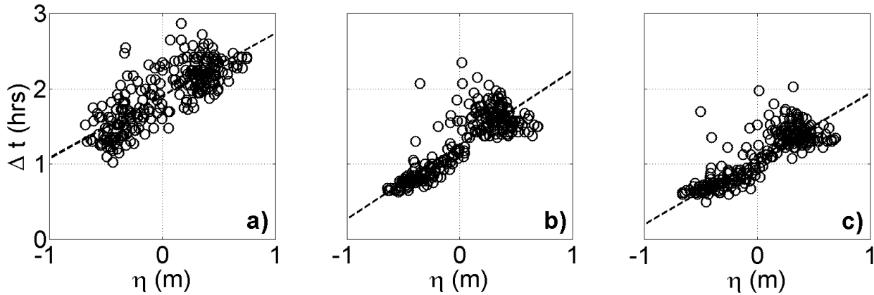
Figure 8. The reflective time lag estimated from daily high tide and low tide maxima and minima for three stations longitudinally deployed through the channel in Elkhorn Slough, CA. Dashed line represents the best-fit line estimated with linear regression. The linear slopes are 0.83, 0.99, and 0.87 and the R^2 -values are 0.59, 0.69, and 0.60 for the three stations.
