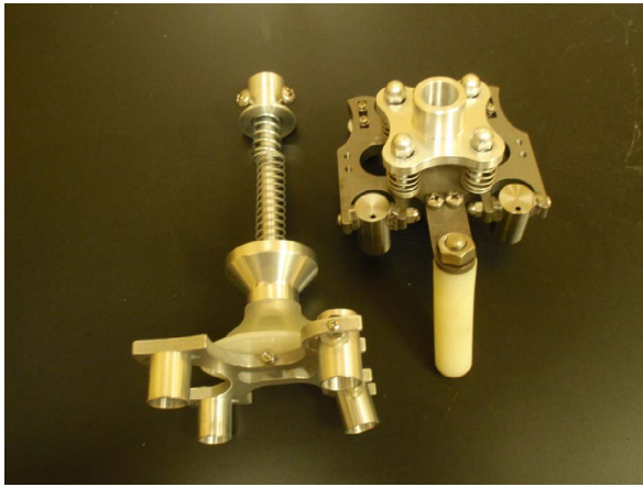
Figure 2: the new 1- and 4-spring shock absorbing robot (left) and the GL (giraffe leg technique) with 3 studs (right)
