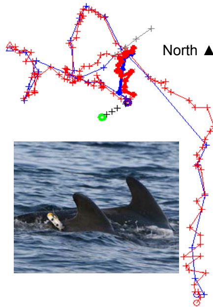
Figure 2. Detailed movement track of tagged whale gm13_169a. The visual sightings are shown as blue crosses, and fixes from the GPS logger are shown in red. Bold sections of the whale track are positions during playback of killer whale sounds. The position of the playback vessel is shown by green and blue circles with x's showing the drifting motion of the playback boat. Note the very high number of fixes from the GPS logger, and the close match between visual and GPS tracks of the whale. Inset box shows the Dtag version 2 with GPS logger (small antenna) attached to a pilot whale.
