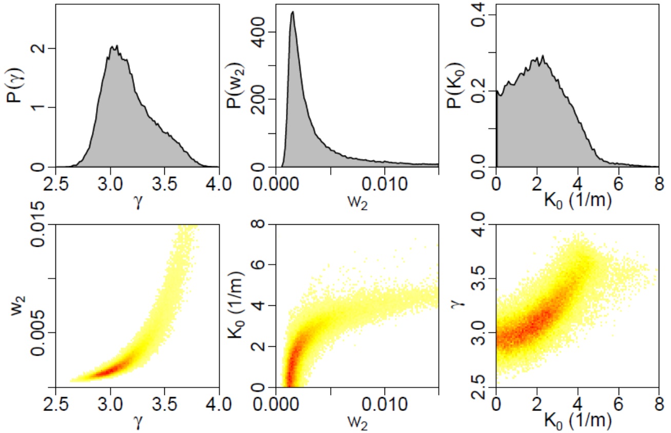
Figure 3: The 1D (top-row) and 2D (bottom row) marginal posterior probability distributions of the scattering parameters (scaled so each distribution has the same area).
