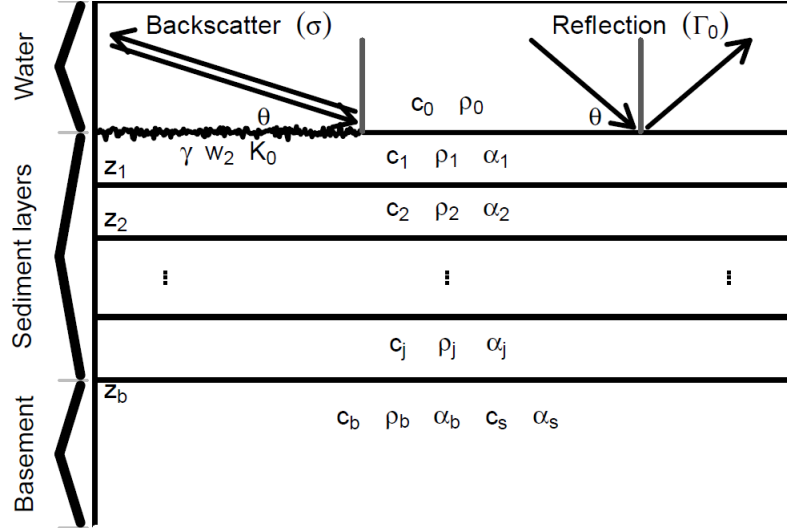
Figure 1: Schematic diagram of the monostatic scattering kernel and reflection coefficient forward models.
