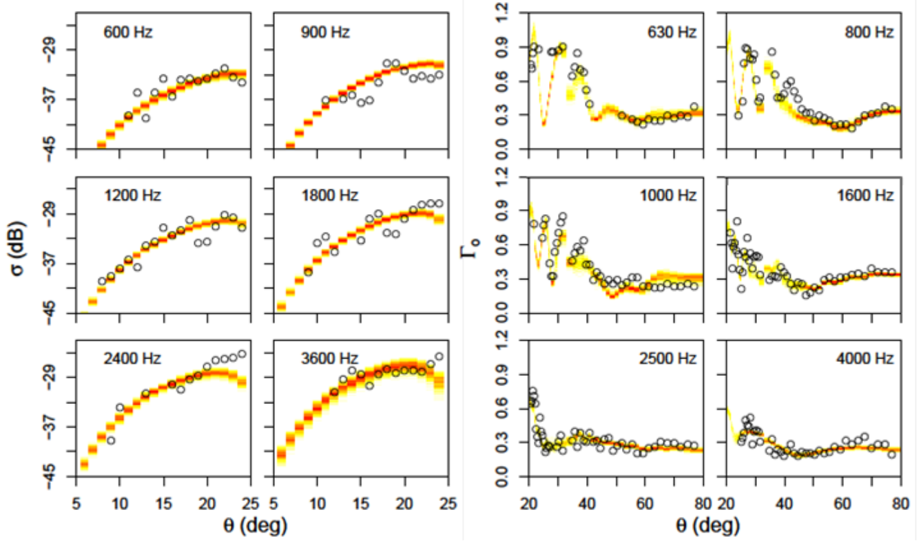
Figure 2: Left, the measured scattering data (o), and right, reflection data (o) as a function of angle and frequency with marginal predicted values.
