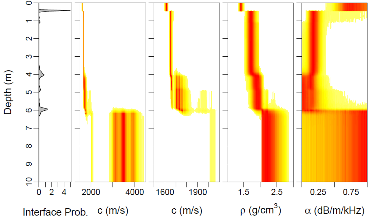
Figure 4: Marginal posterior profiles for geoaoustic properties from joint scattering reflection inversion. Plot boundaries correspond to prior bounds.
