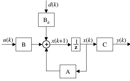
Figure 4. System representation.
