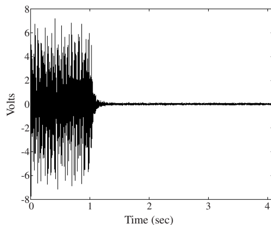
Figure 10. Uncontrolled response and MIMO controlled response of five disturbance frequencies (repetition 10).
