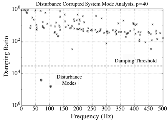
Figure 5. Clear box system identification, analysis of modes.
