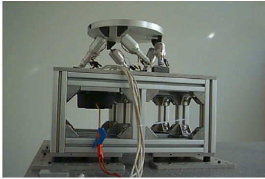
Figure 1. UQP and satellite bus mockup. (This figure is in colour only in the electronic version)
