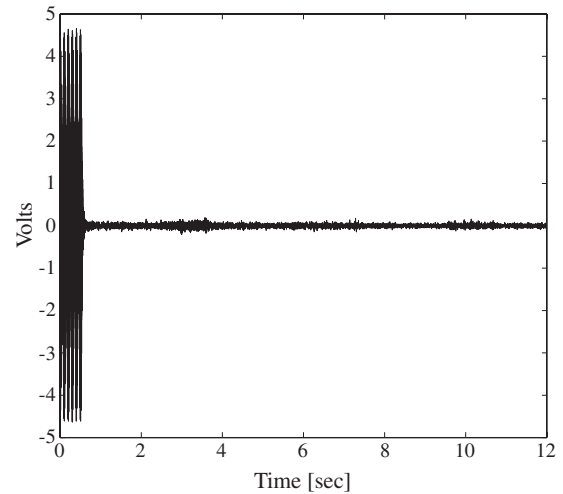
Figure 9. Uncontrolled response and clear box adaptive basis method response, one varying frequency.
