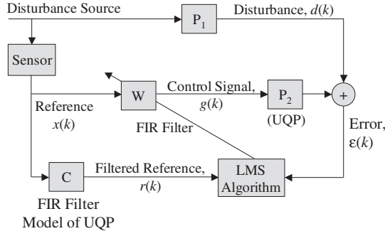
Figure 3. Multiple error least mean square algorithm.
