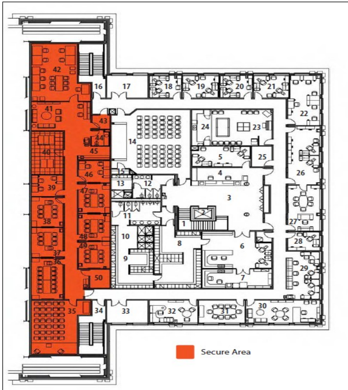
Second Floor, Prototype Squadron Operations Facility Used as template for designing layout of eQUEST model
